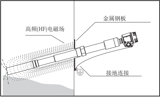
塑料壁料仓
