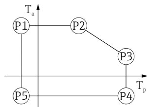
39 铝外壳，带涂层；过程温度范围：-20 ... +200 °C (-4 ... +392 °F)
