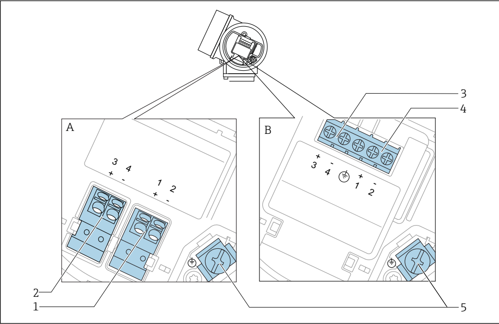
18 接线端子分配: 两线制; 4...20 mA HART, 4...20 mA
