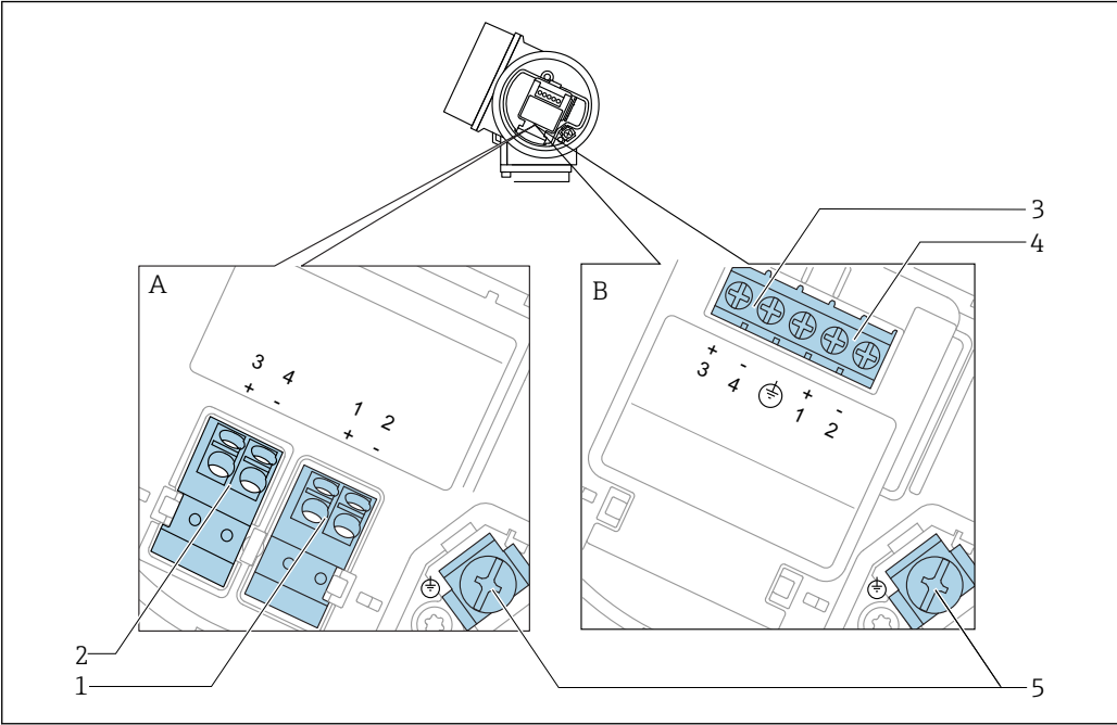
8 接线端子分配: PROFIBUS PA / FOUNDATION Fieldbus
