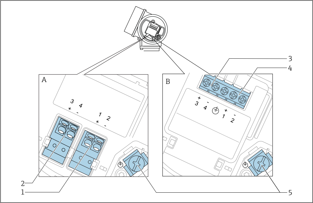
14 接线端子分配: PROFIBUS PA / FOUNDATION Fieldbus
