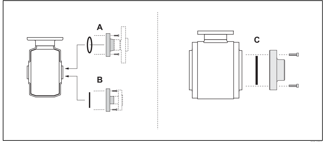
图 20: Promag H 传感器的过程连接: DN 2...25 (1/12"..."1") / DN 40...100 (1 1/2"..."4")
