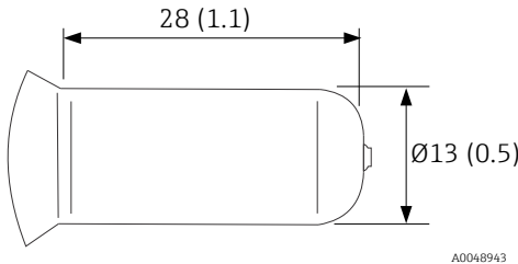
Figure 3. Tip of 2" Rxn-41 probe. Dimensions: mm (in)
