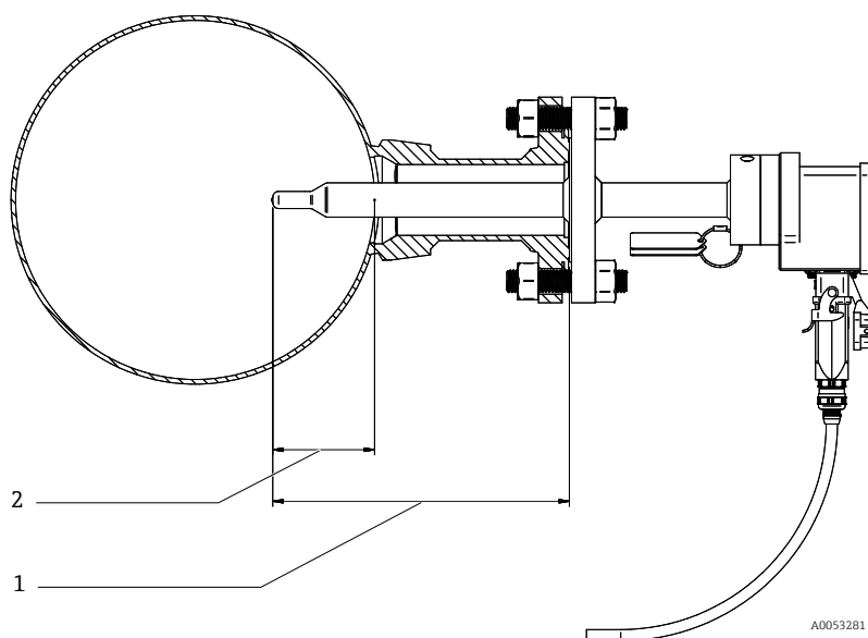
Figure 2. Rxn-41 probe installation for LNG Service
