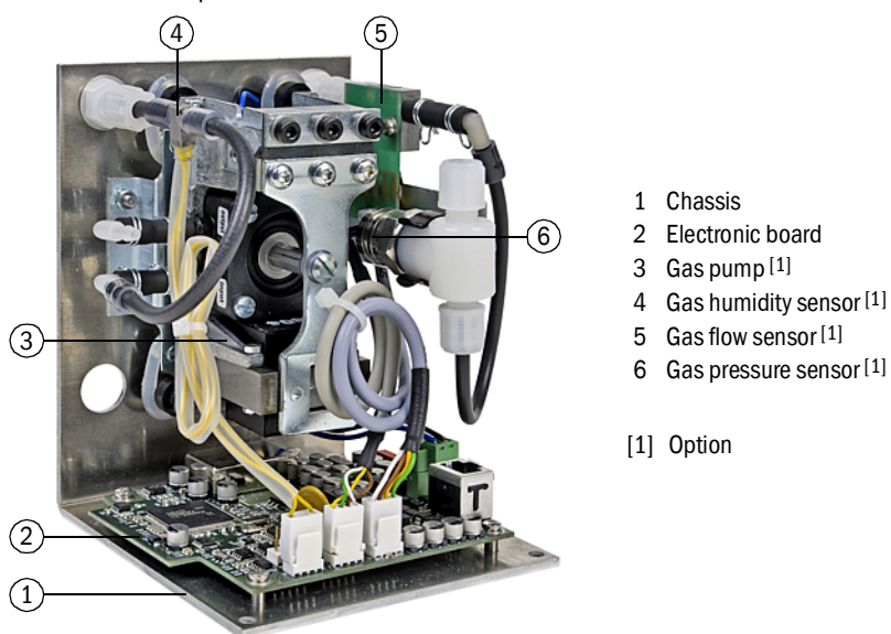
Gas module components
