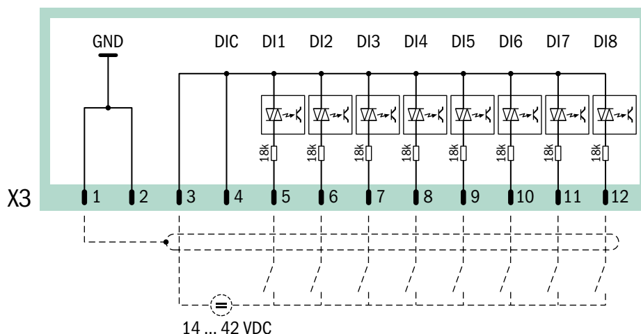
Plug connector X3 (digital inputs)
