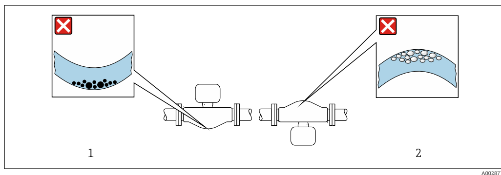
14 Orientation of sensor with curved measuring tube
