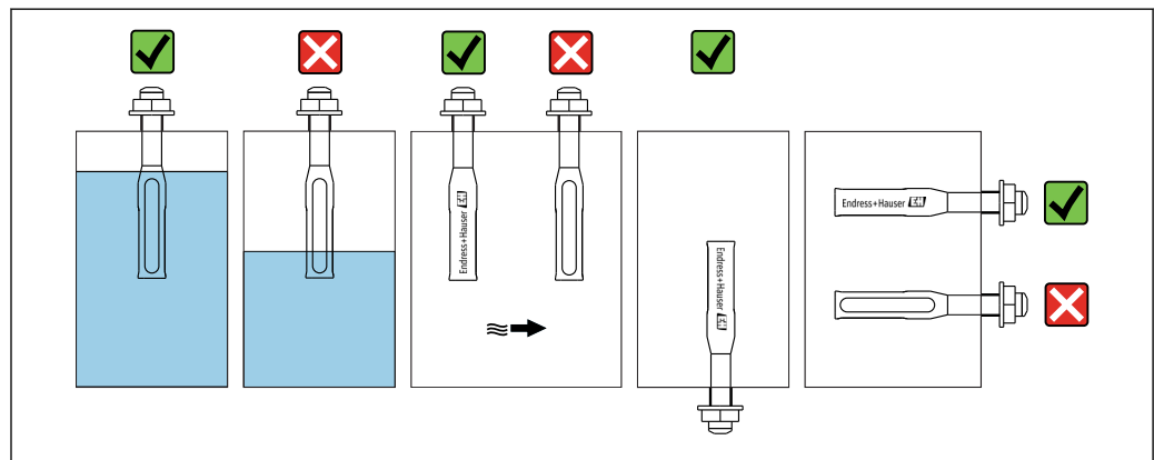
5 Orientation of Tegwave I
