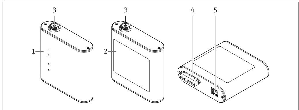
2 Transmitter versions
