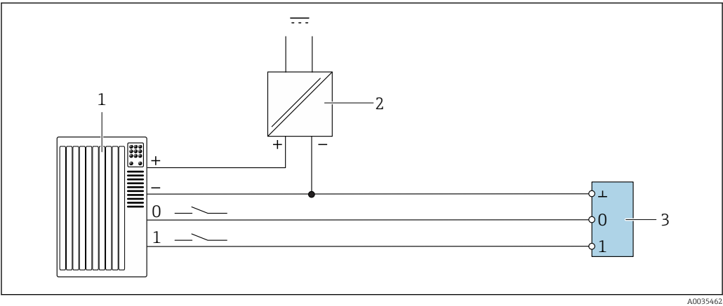
12 Connection example for the digital input 1 Automation system with switch input (e.g. PLC) 2 Power supply 3 Transmitter
