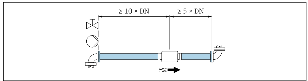
6 Inlet and outlet runs
