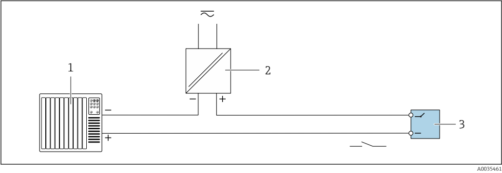
11 Connection example for relay output, passive 1 Automation system with switch input (e.g. PLC) 2 Power supply: max. 50 V AC/DC 3 Transmitter
