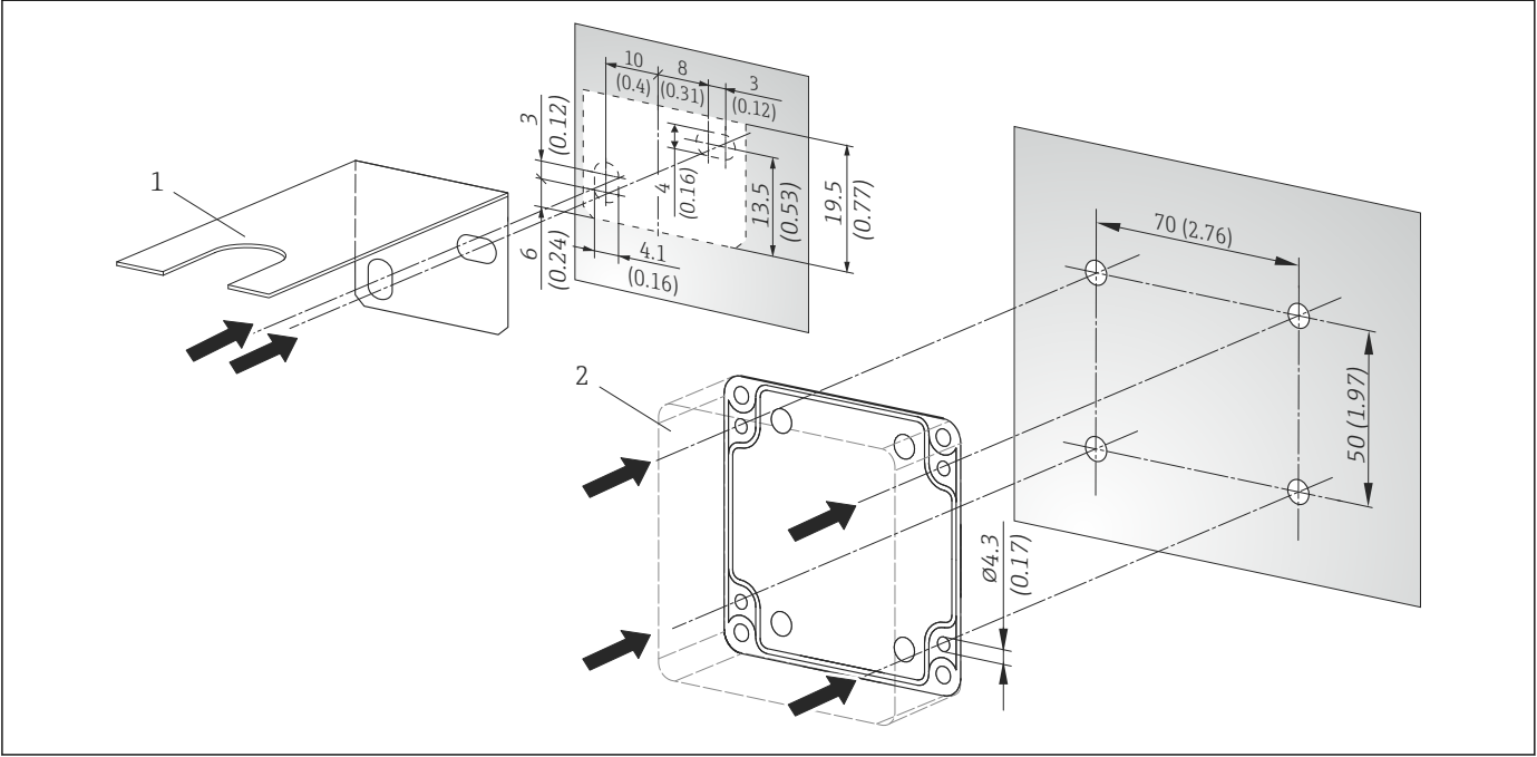
6 Drilling templates for wall mounting. Dimensions in mm (in) 1 Mounting bracket for mounting with terminal head 2 Plastic housing
