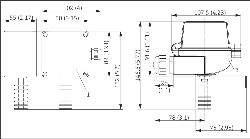
7 Dimensions of the thermometer 1 With plastic housing 2 With terminal head
