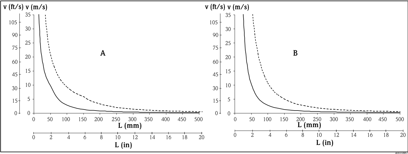
Permitted flow velocity - Insert diameter 3 mm (0.12 in) — - Insert diameter 6 mm (0.24 in) - - - -
