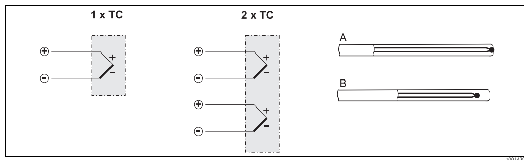
Wiring diagram
