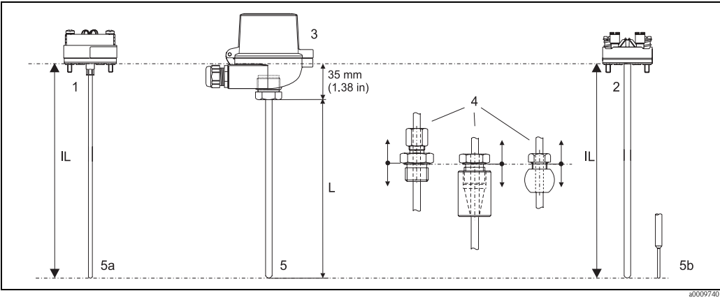
Equipment architecture of the Omnigrad T TR24
