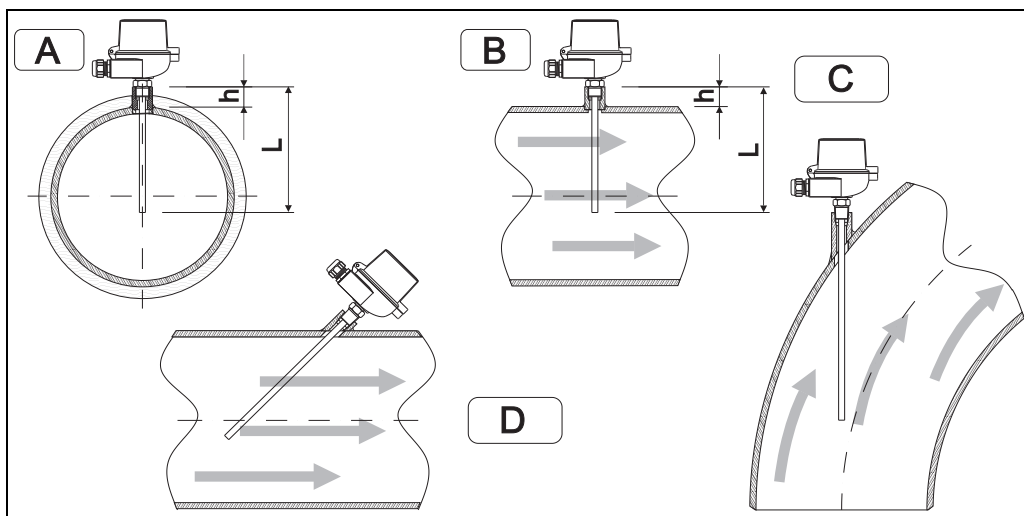
Installation examples
