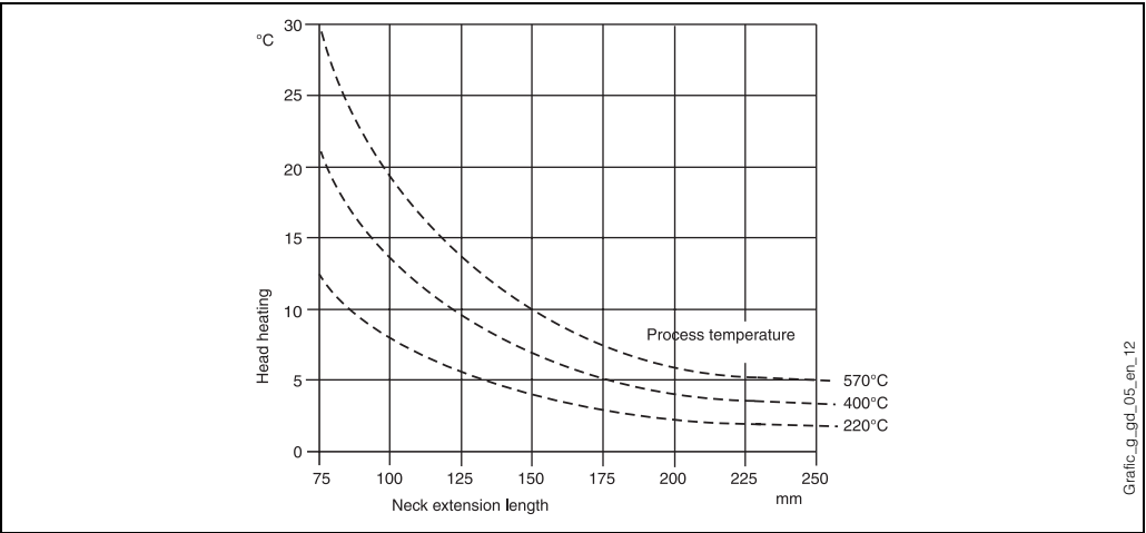
Fig. 4: Heating of the head consequent to the process temperature
