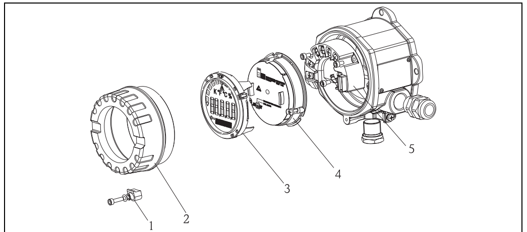
Fig. 3: Turning the display
