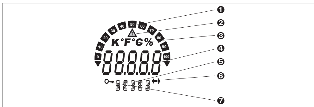
Fig. 9: LC display of the field transmitter (illuminated, can be plugged in 90° stages)
