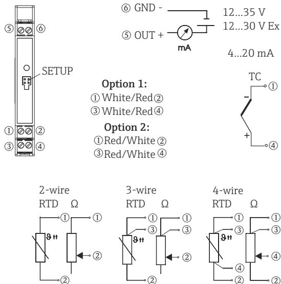
3: Terminal layout
