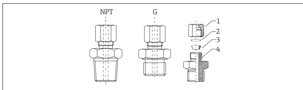
3 Compression fitting
