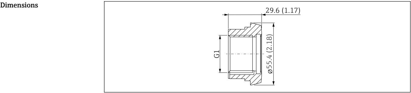
56 Dimensions of process adapter DIN11851 DN40 (G1). Unit of measurement mm (in)
