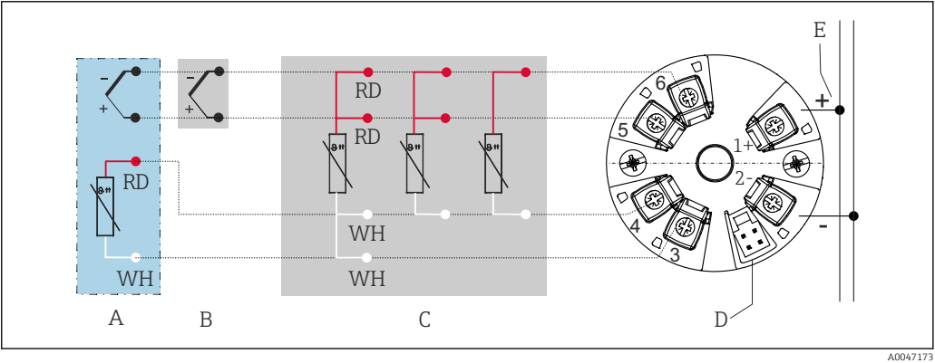
2 Head mounted transmitter TMT31 (single input)
