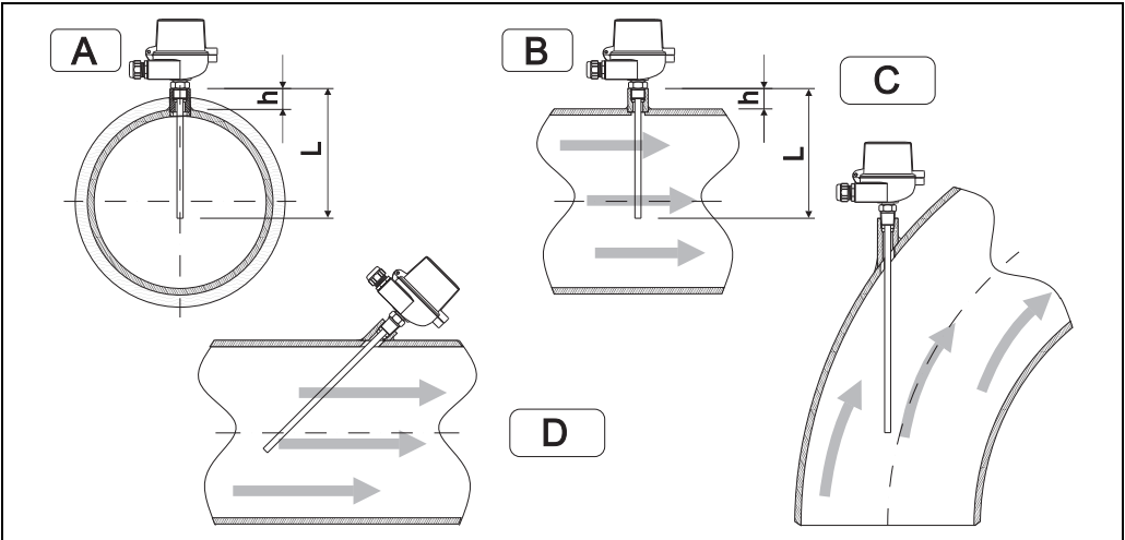
Installation examples A - B: In pipes with a small cross section the sensor tip should reach or extend slightly past the center line of the pipe (= L). C - D: Tilted installation.
