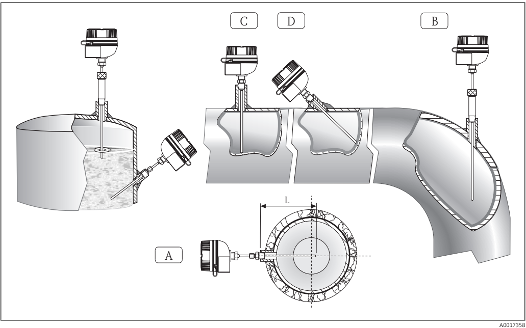
6 Thermometer installation
