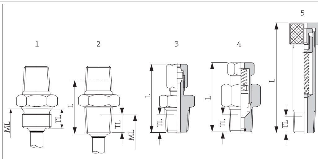
5 Available process connections
