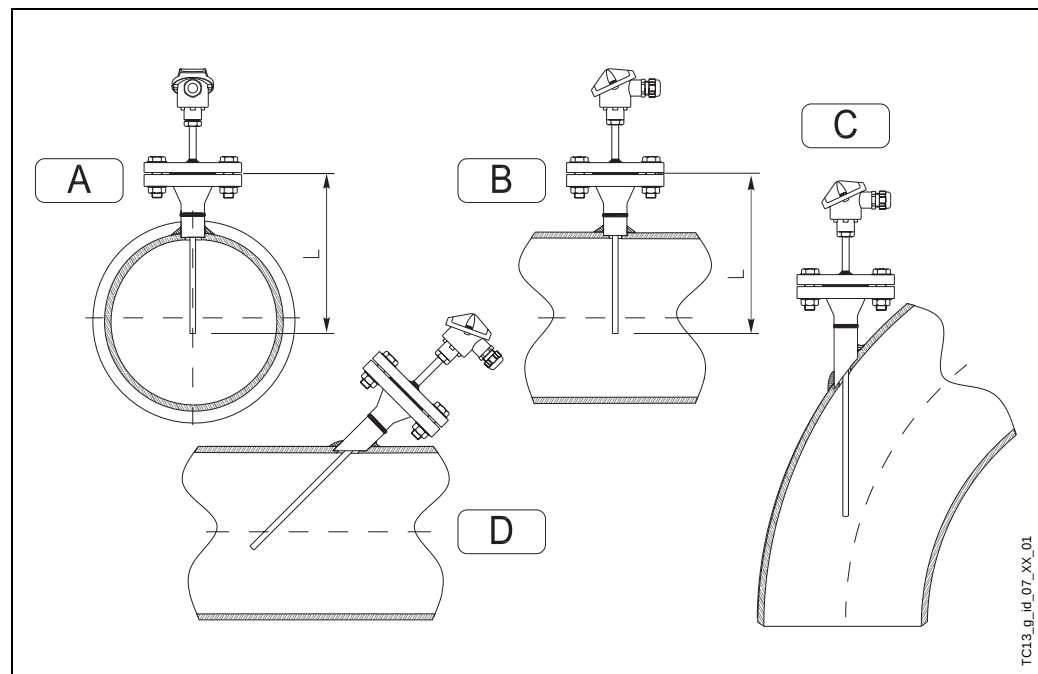
Fig. 4: Installation examples
