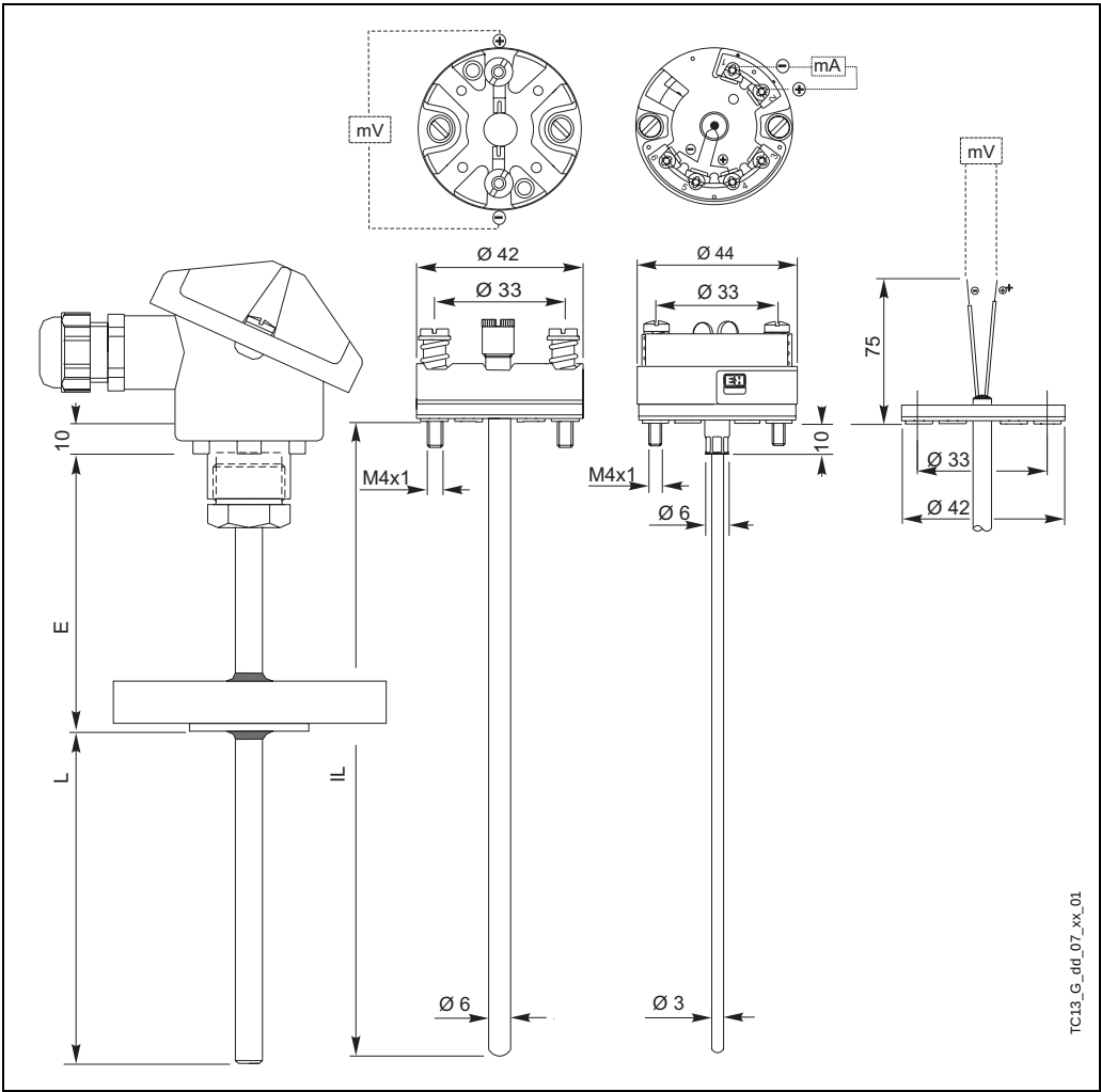
Fig. 11: Functional components
