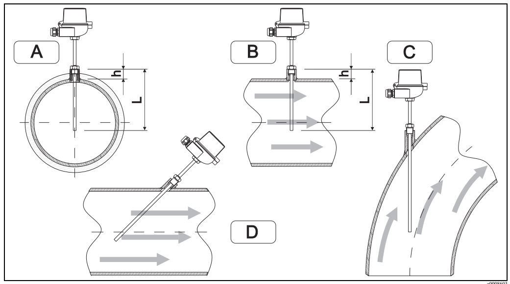
Installation examples
