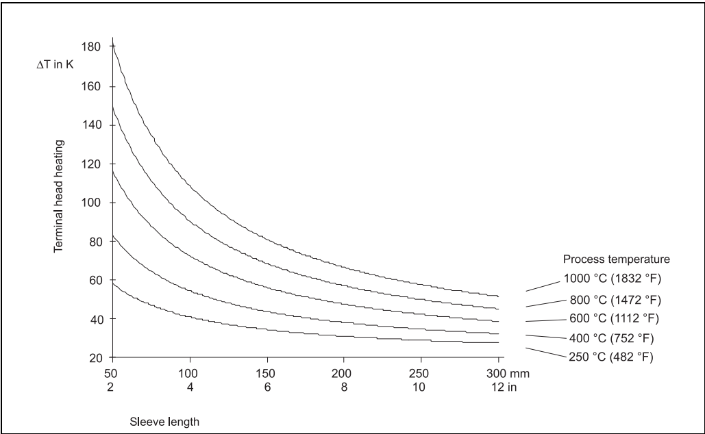
Heating of the terminal head consequent to the process temperature Temperature in terminal head = ambient temperature 20 °C (68 °F) + ΔT Sleeve-Ø = 3/4" schedule 40
