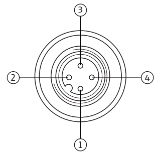
Fig. 7-3: PIN assignment of M12 socket
