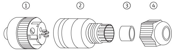
Fig. 7-2: Disassembling and assembling the M12 socket
