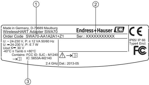
Fig. 2-1: Nameplate (example)
