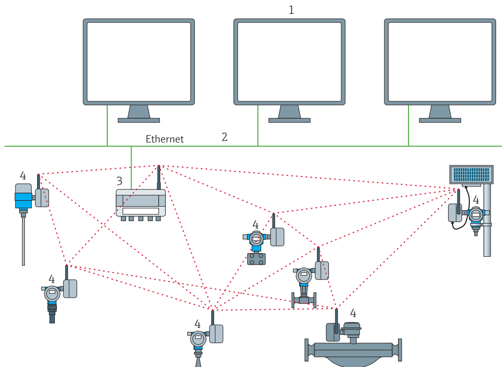
Fig. 3-1: WirelessHART network
