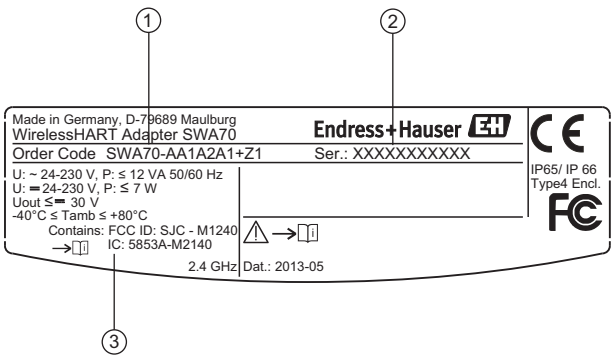
Fig. 2-1: Nameplate (example)
