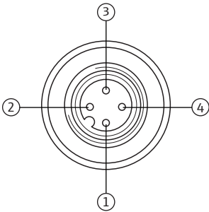
Fig. 6-3: PIN assignment of M12 socket
