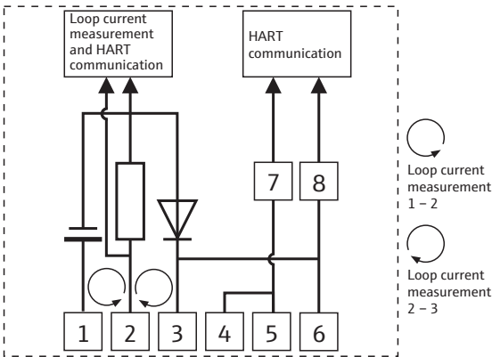
Fig. 5-3: Assignment of terminals
