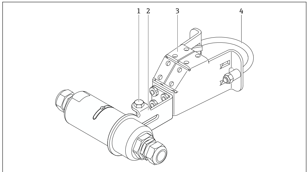
8 FieldPort SWA50 mounted via optional mounting bracket
