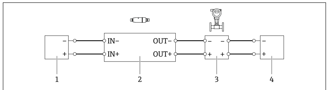
12 Electrical connection for 4-wire HART field devices with passive current output (optional grounding not shown)
