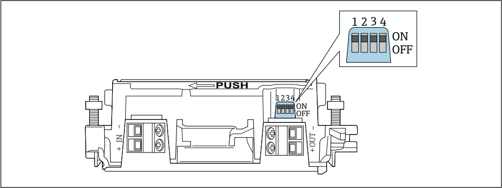
20 DIP switches for hardware-locking of functions
