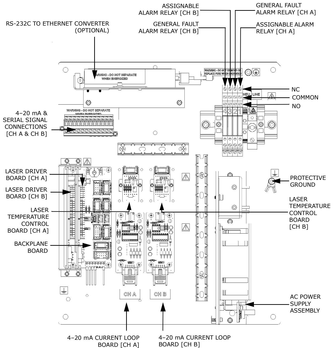
Figure 1-7 Electronics control board (AC) for dual-channel systems (SS3000e) with RS-232C to Ethernet converter
