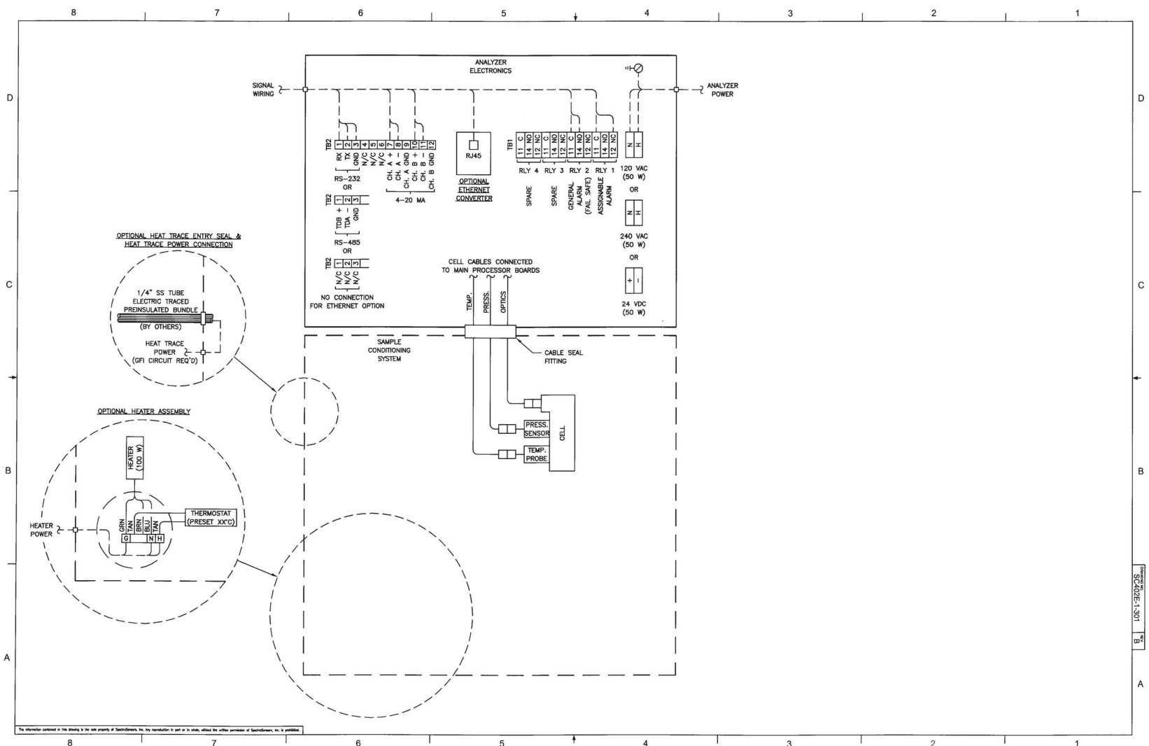
Figure A-3 SS500e/SS2000e analyzer system power and signal wiring diagram
