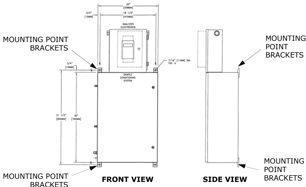
Figure 3-1 Gas analyzer carrying points/methods
