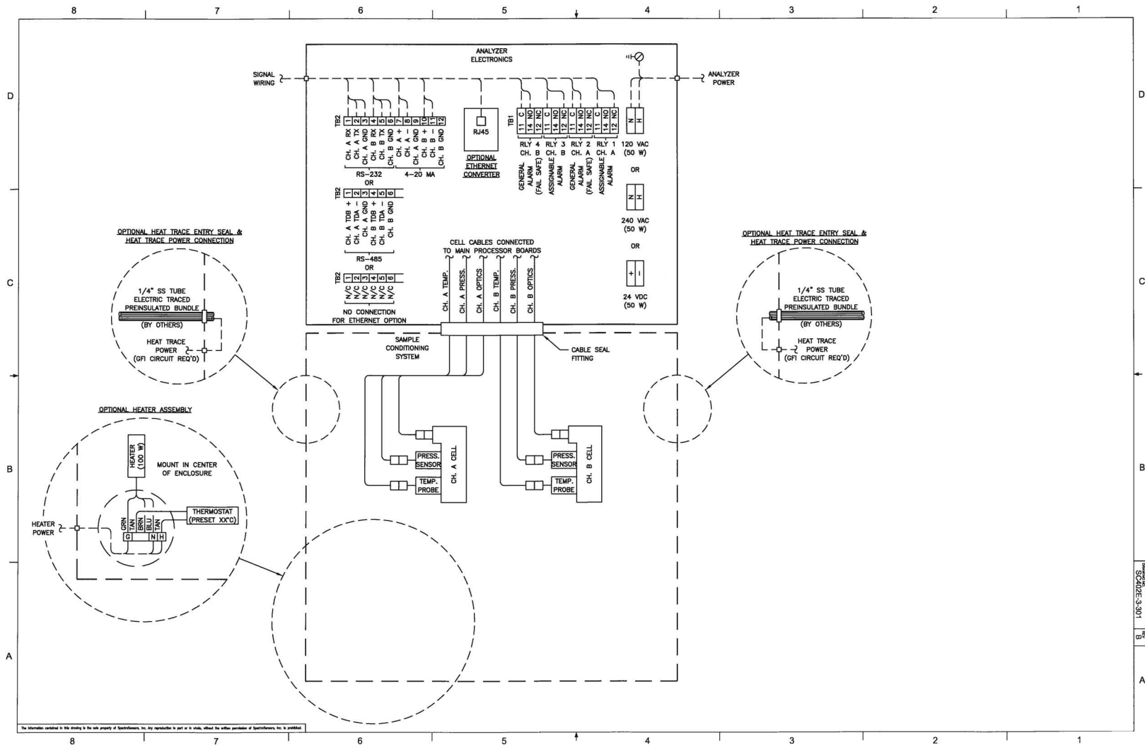
Figure A-10 SS3000e dual stream analyzer system power and signal wiring
