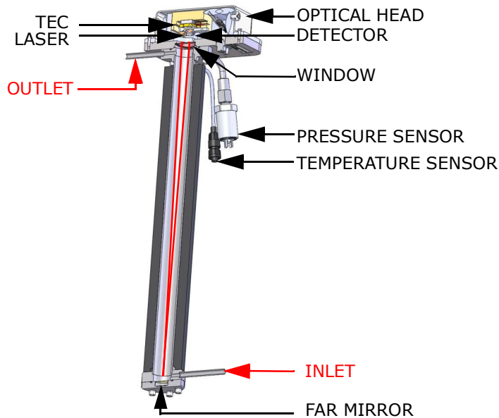
Figure 1-1 Schematic of a typical laser diode absorption spectrometer
