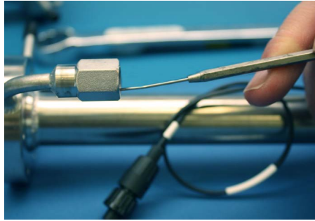
Figure B-7 Removing excess seal tape from flange
