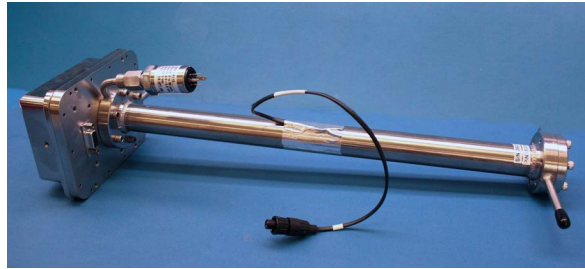
Figure B-5 Removed measurement cell with pressure sensor face up
