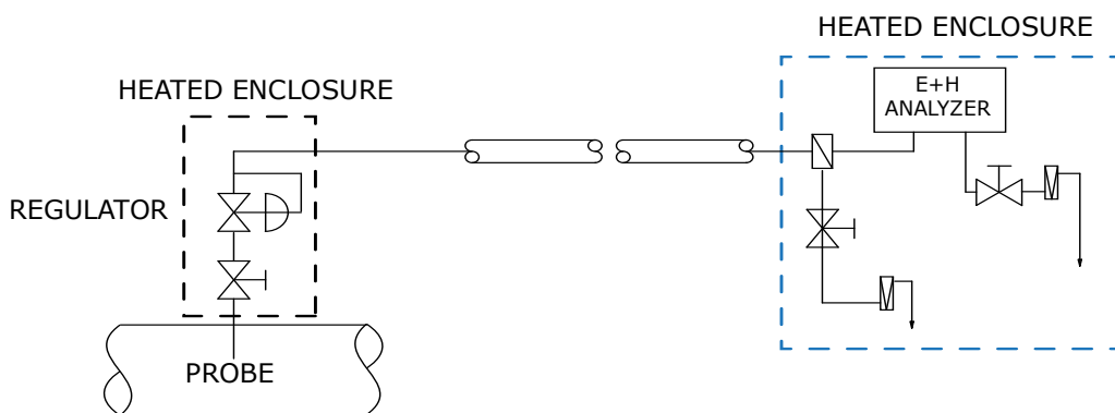
Figure 4–1 Probe to gas analyzer interface
