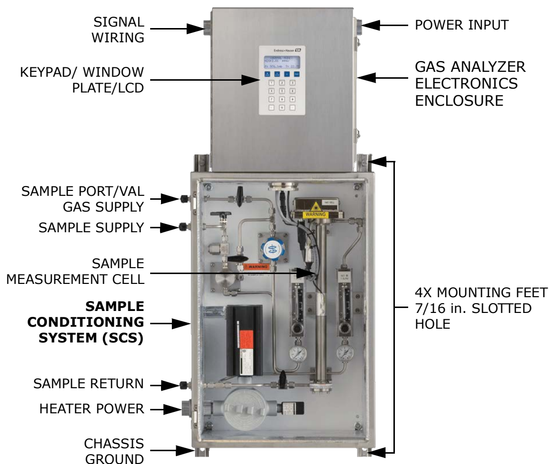
Figure 1–5 SS500e/SS2000e architecture overview
