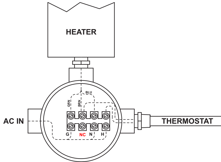
Figure 3-3 AC connection terminal block for enclosure heater
