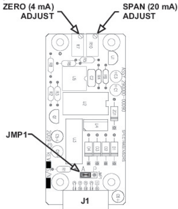
Figure 3–7 4–20 mA output board
