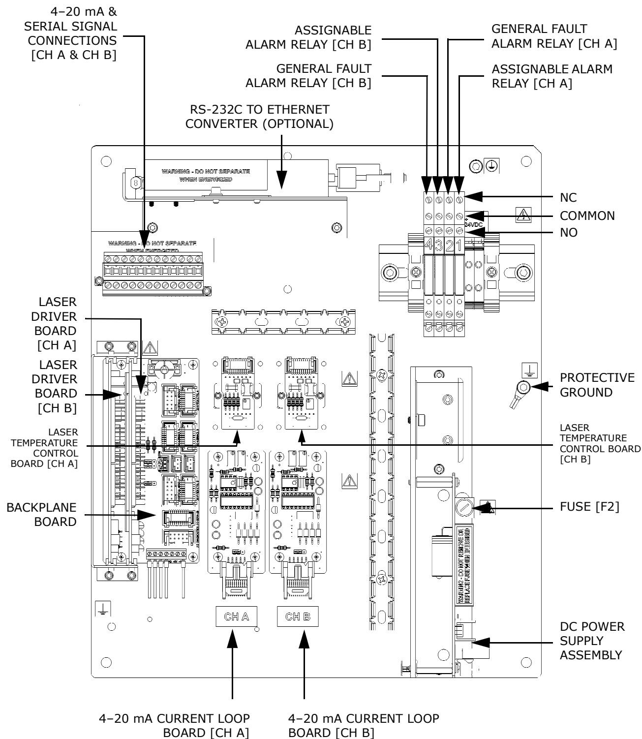
Figure 1-8 Electronics control board (DC) for dual-channel systems (SS3000e) with RS-232C to Ethernet converter
