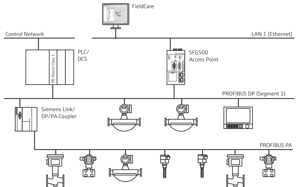
Fig. 4-1: Architecture for Siemens coupler/link
