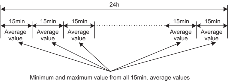
Fig. 1: Recording the highest and lowest values over one day (x = 15 min.)
