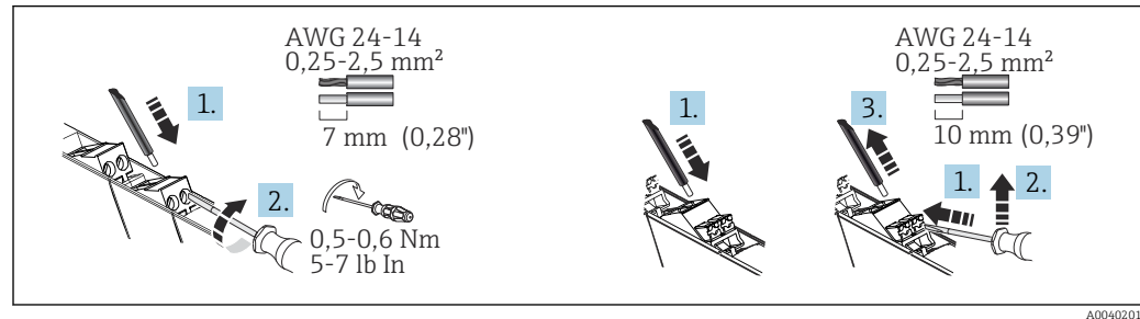
5 Electrical connection using screw terminals (left) and push-in terminals (right)
