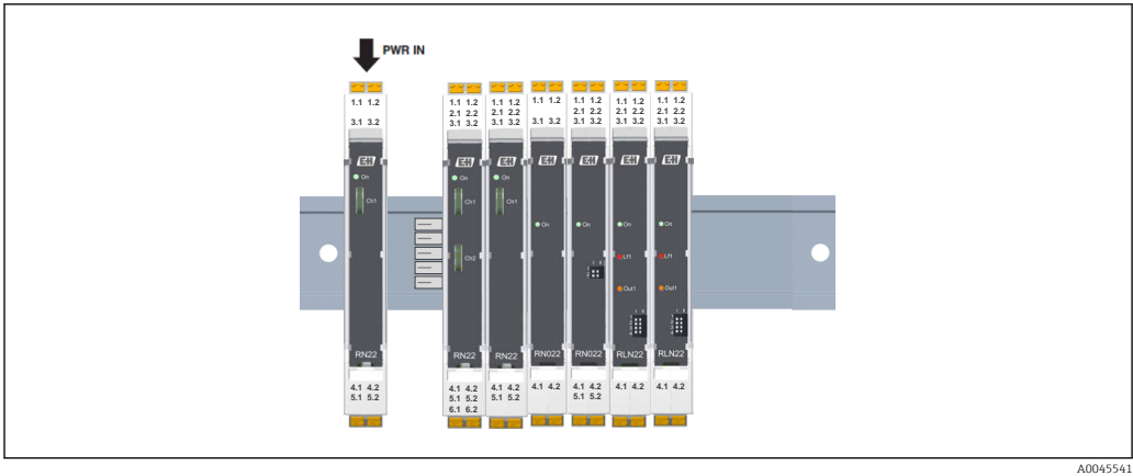
12 Direct power feed-in at any device in the group
