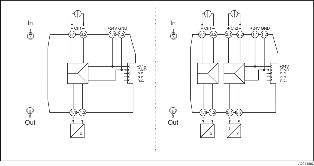
6 Terminal assignment of RNO22: 1-channel version (left), 2-channel version (right)
