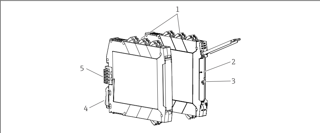
11 Display and operating elements 1 Plug-in screw or push-in terminal with integrated test socket 2 Green LED "PWR" power supply 3 DIP switches (only on 1-channel version) 4 DIN rail clip for DIN rail mounting 5 DIN rail bus connector (optional)
