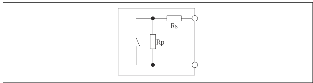
22 Resistance circuit for line monitoring (short-circuit and line break)
