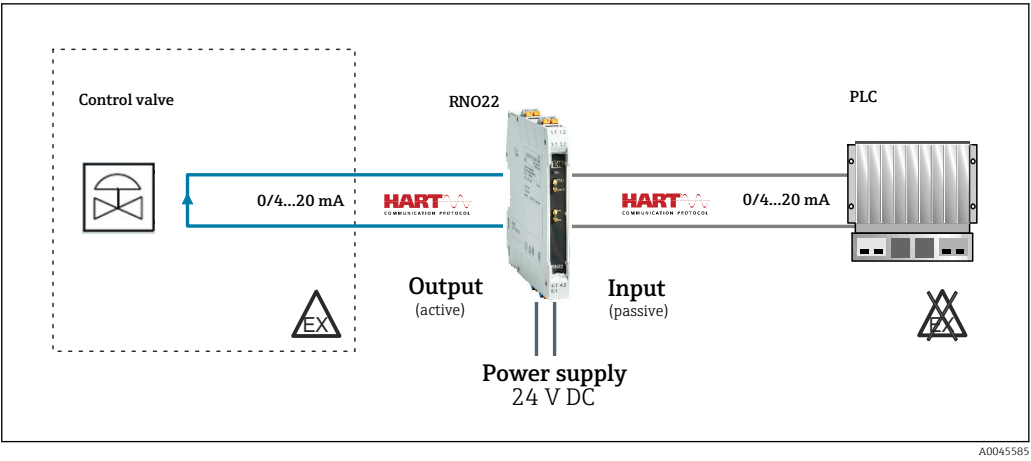
23 Control valve activation in the hazardous area with an RNO22 output isolating amplifier
