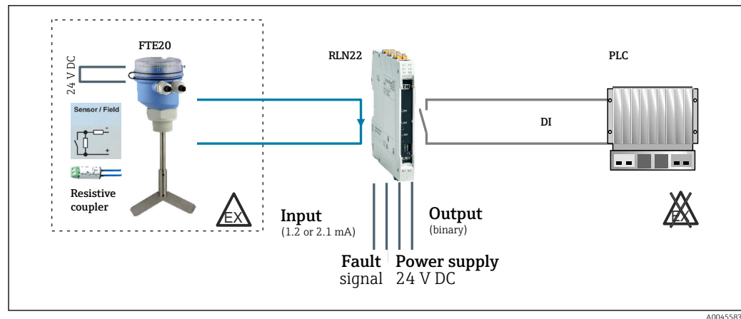
21 NAMUR limit detection with FTE20 paddle switch with line monitoring in the hazardous area
