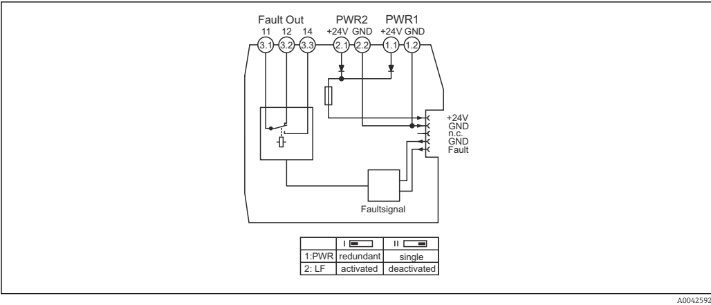
6 RNF22 terminal assignment: power and error message module
