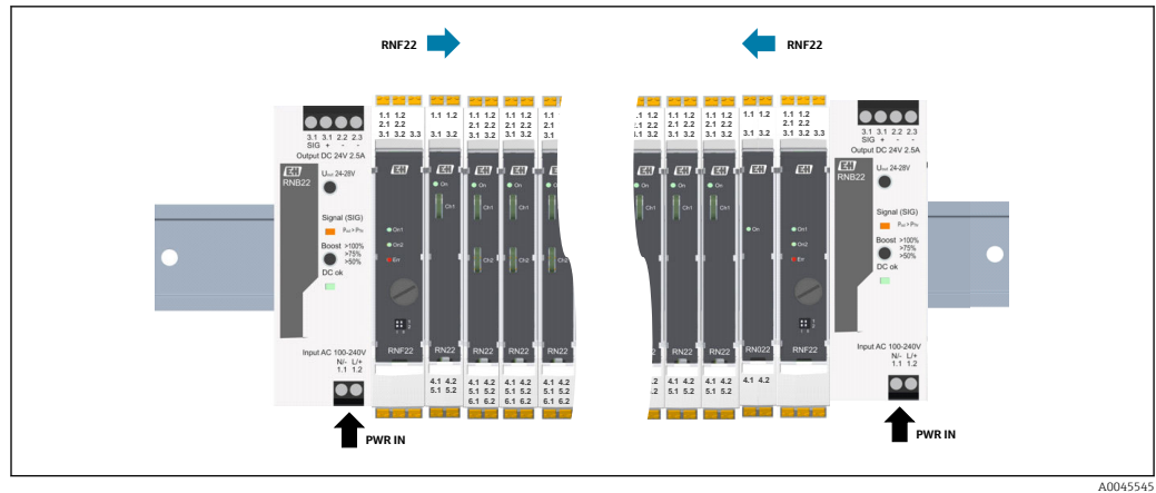
15 Example of power feed-in via two RNF22 power modules
