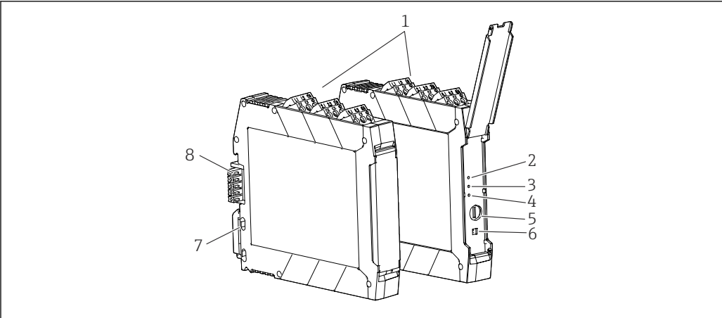
11 Display and operating elements
