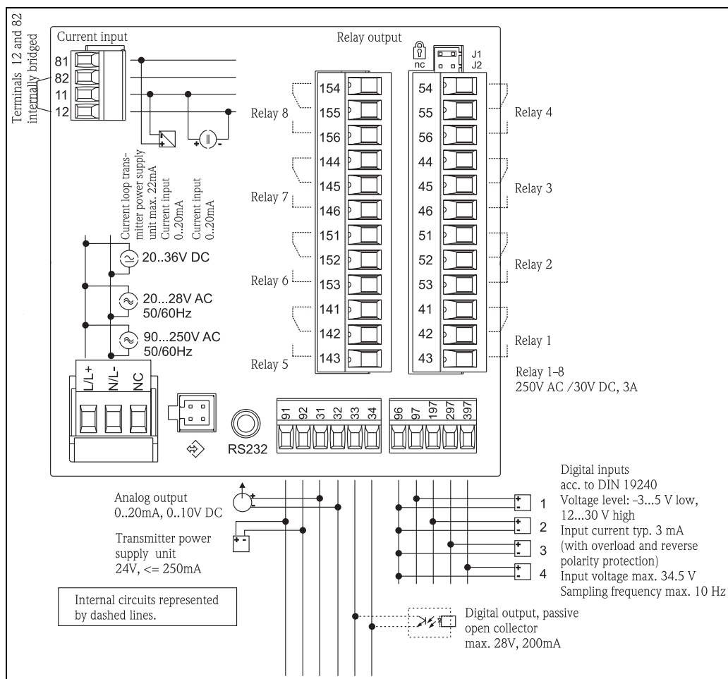
Terminal assignment of process display unit
