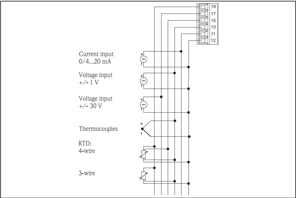
Universal input terminal assignment
