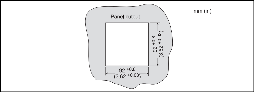
Panel cutout
