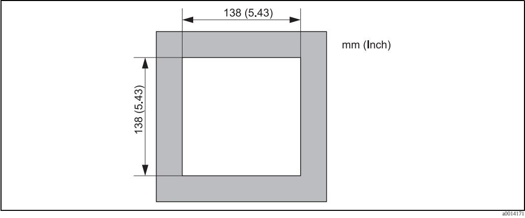
Panel cutout
