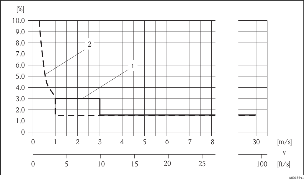
8 Example for max. measured error (volume flow) in % o.r. 1 Standard (order code for "Calibration flow", option 1 "Operable flow range 30 : 1") 2 Optional (order code for "Calibration flow", option 2 "Operable flow range 100 : 1")
