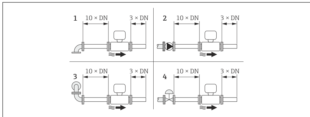
10 Two-path version: minimum inlet and outlet runs with various flow obstructions
