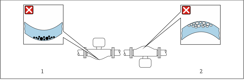
☒ 13 Orientation of sensor with curved measuring tube 1 Avoid this orientation for media with entrained solids: Risk of solids accumulating 2 Avoid this orientation for outgassing media: Risk of gas accumulating
