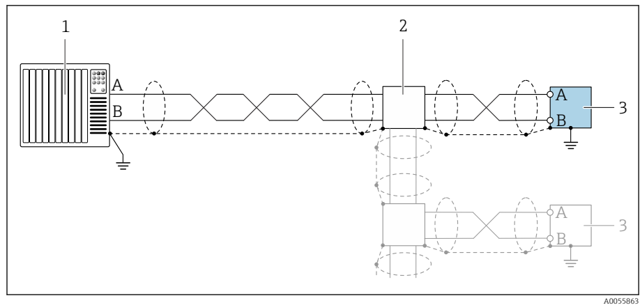
4 Connection example for Modbus RS485
