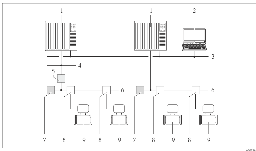
22 Options for remote operation via FOUNDATION Fieldbus network
