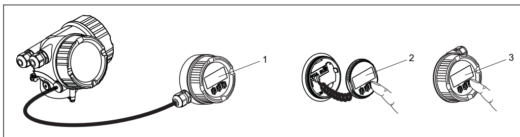
19 Operating options via FHX50
