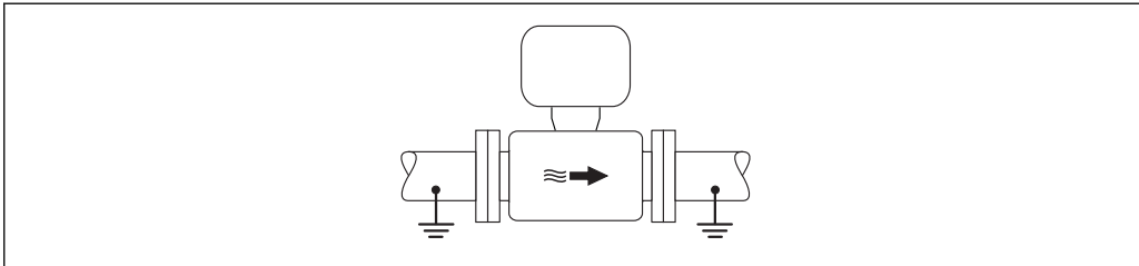
7 Potential equalization via measuring tube
