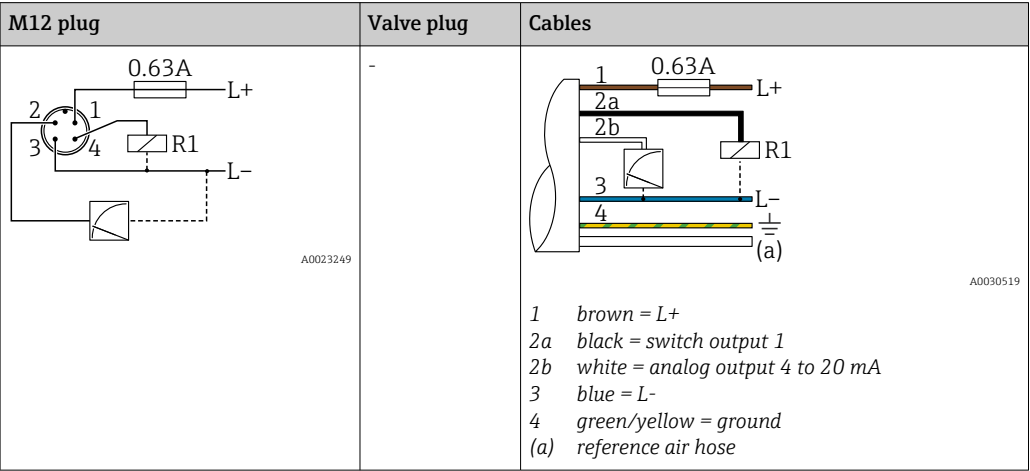
1 x PNP switch output R1 with additional analog output 4 to 20 mA (active)
