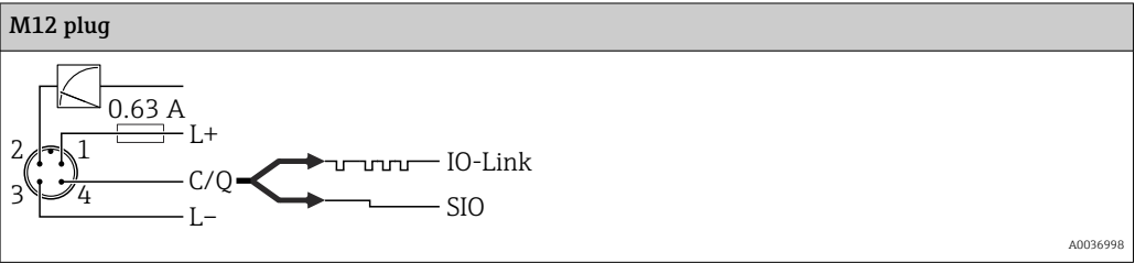
IO-Link: 1 x PNP switch output R1 with additional analog output 4 to 20 mA (active)
