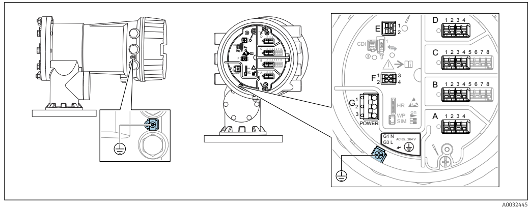
11 Terminal compartment (typical example) and ground terminals
