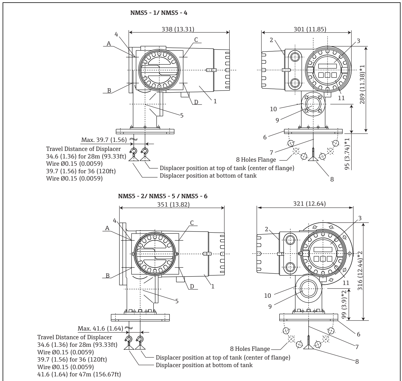
Figure 11: Dimensions of NMS5, Unit of Measurement: mm (in)
