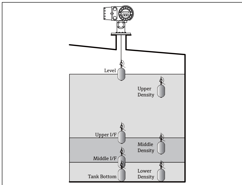
Figure 6: NMS5 with standard level, I/F x 2, Tank bottom and spot density x 3 measurement
