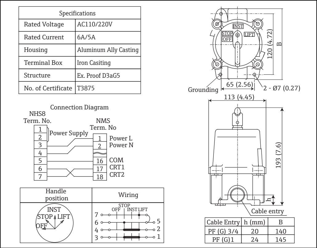
Figure 15: Power and Control Switch, Unit of Measurement: mm (in)
