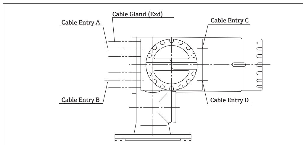
Figure 12: Cable Entries
