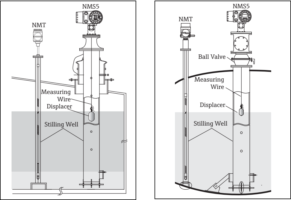
Figure 4: Fixed Roof Tank (Left) / High Pressure Tank (Right)
