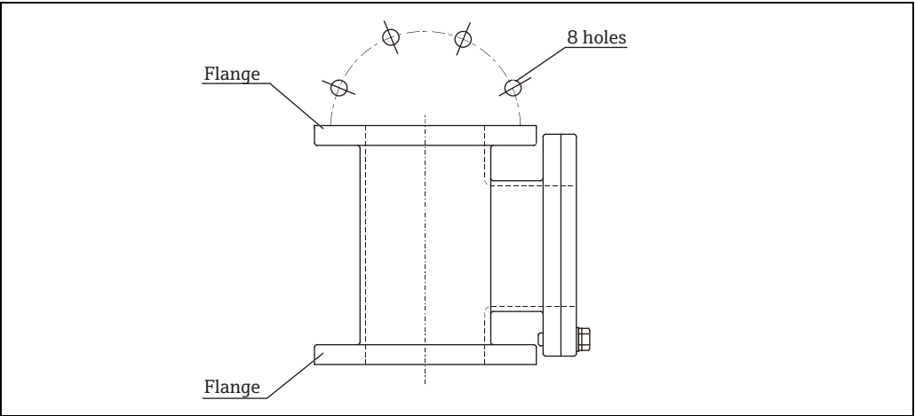
Figure 14: Calibration Chamber, Unit of Measurement: mm (in)
