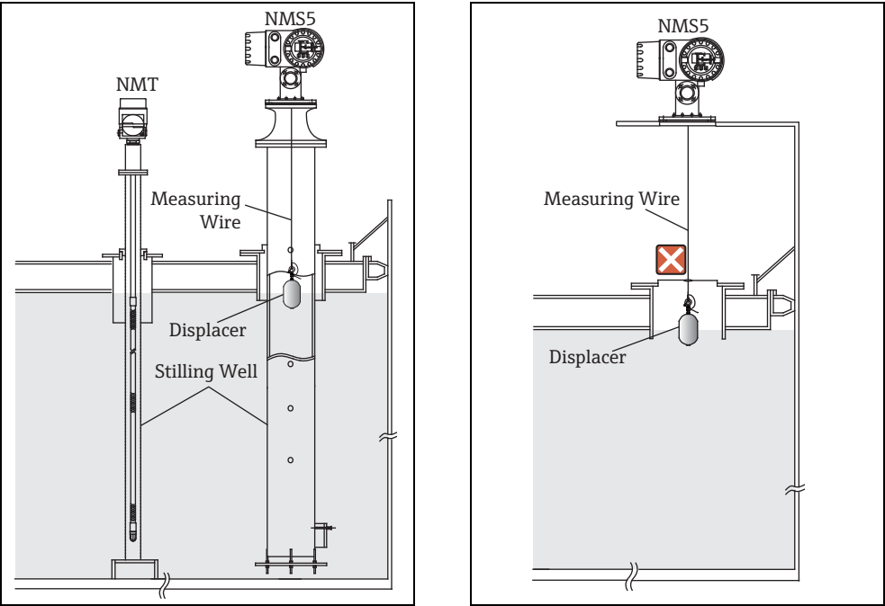
Figure 5: Floating Roof Tank
