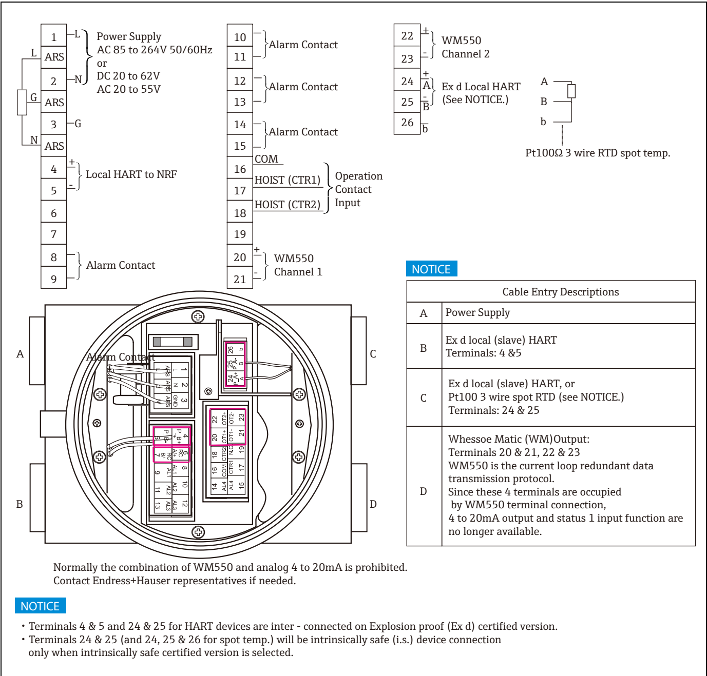
Figure 9: Wiring Sample 2
