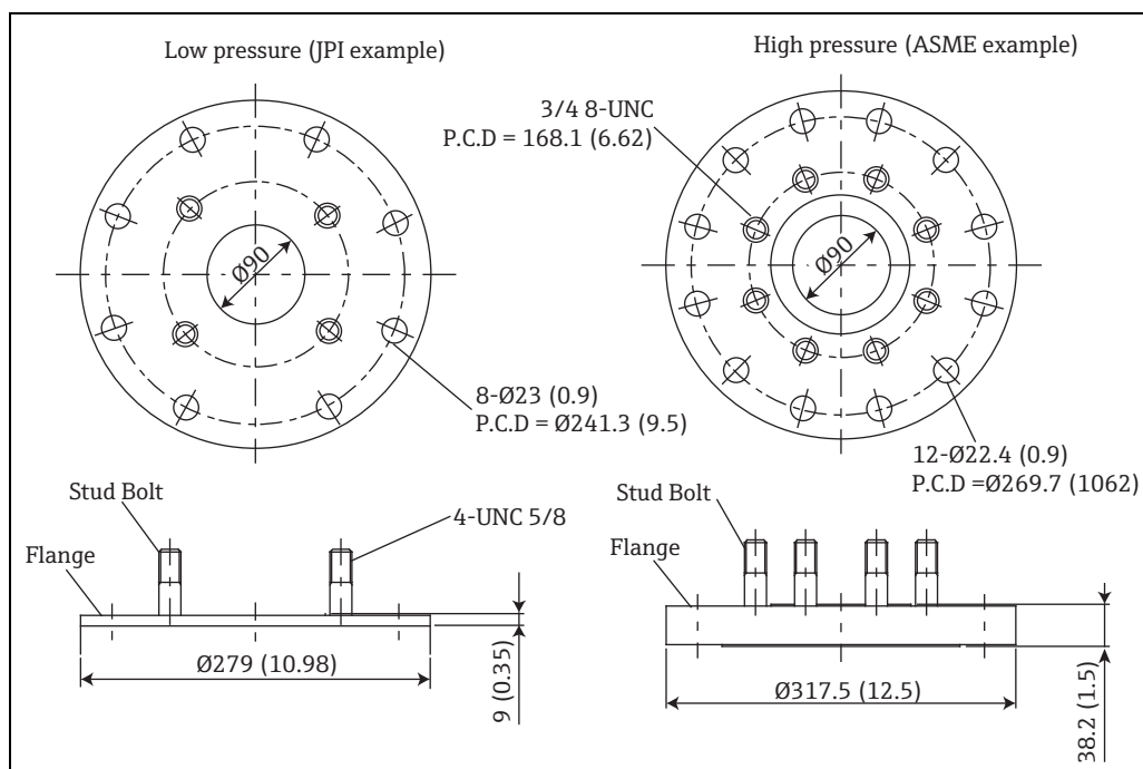
Figure 17: Reducing Flange, Unit of Measurement: mm (in) Use reducing flange when NMS5 connection 80A(30") and mounting nozzle is 150A(6").
