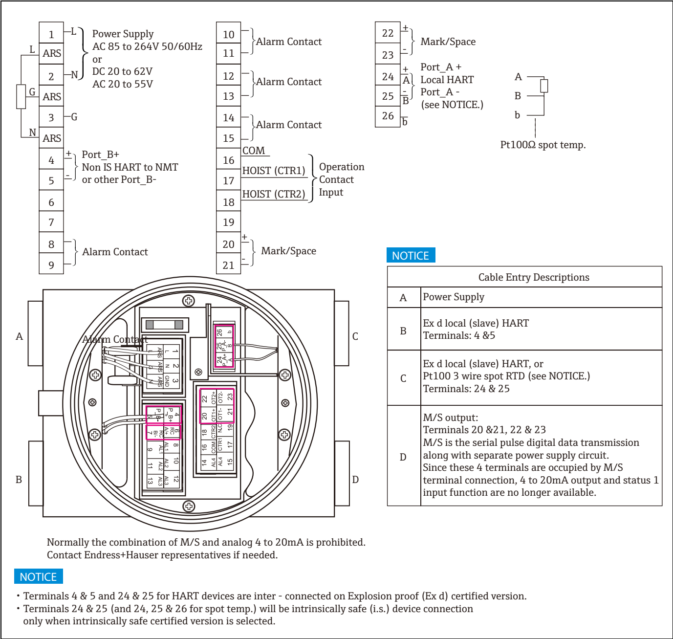
Figure 10: Wiring Sample 3
