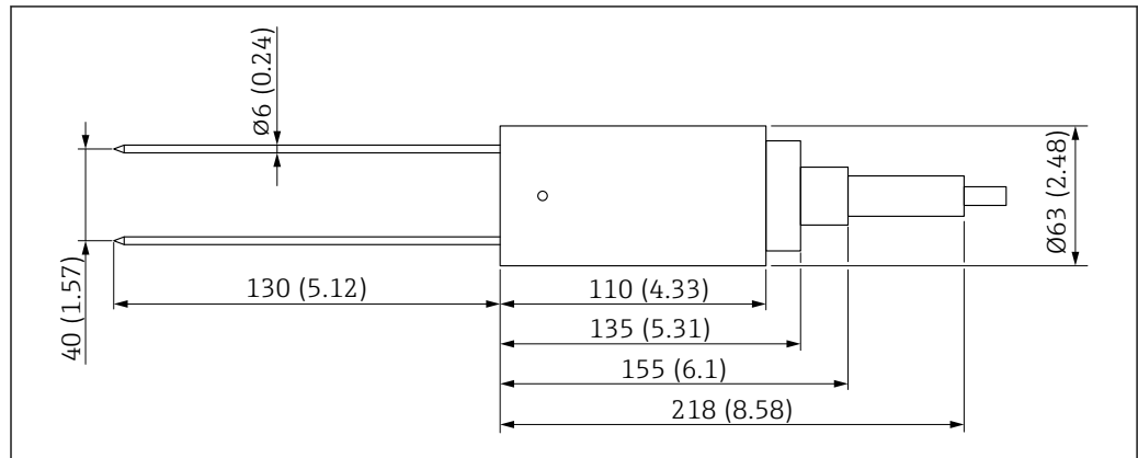
6 Dimensions of S1 two-rod probe. Unit of measurement mm (in)
