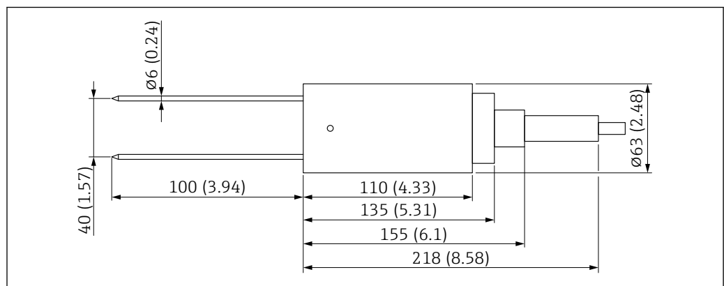
8 Dimensions of S1C two-rod probe. Unit of measurement mm (in)
