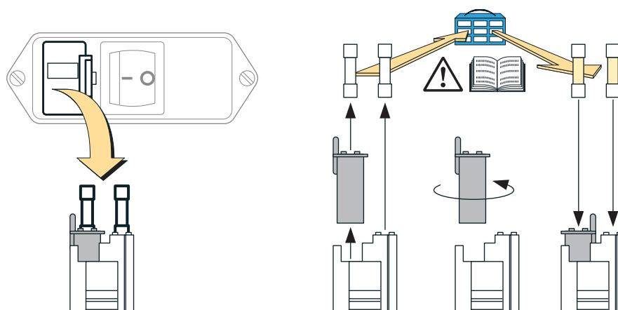
Fig. 33: Power fuses / Changing the required power voltage
