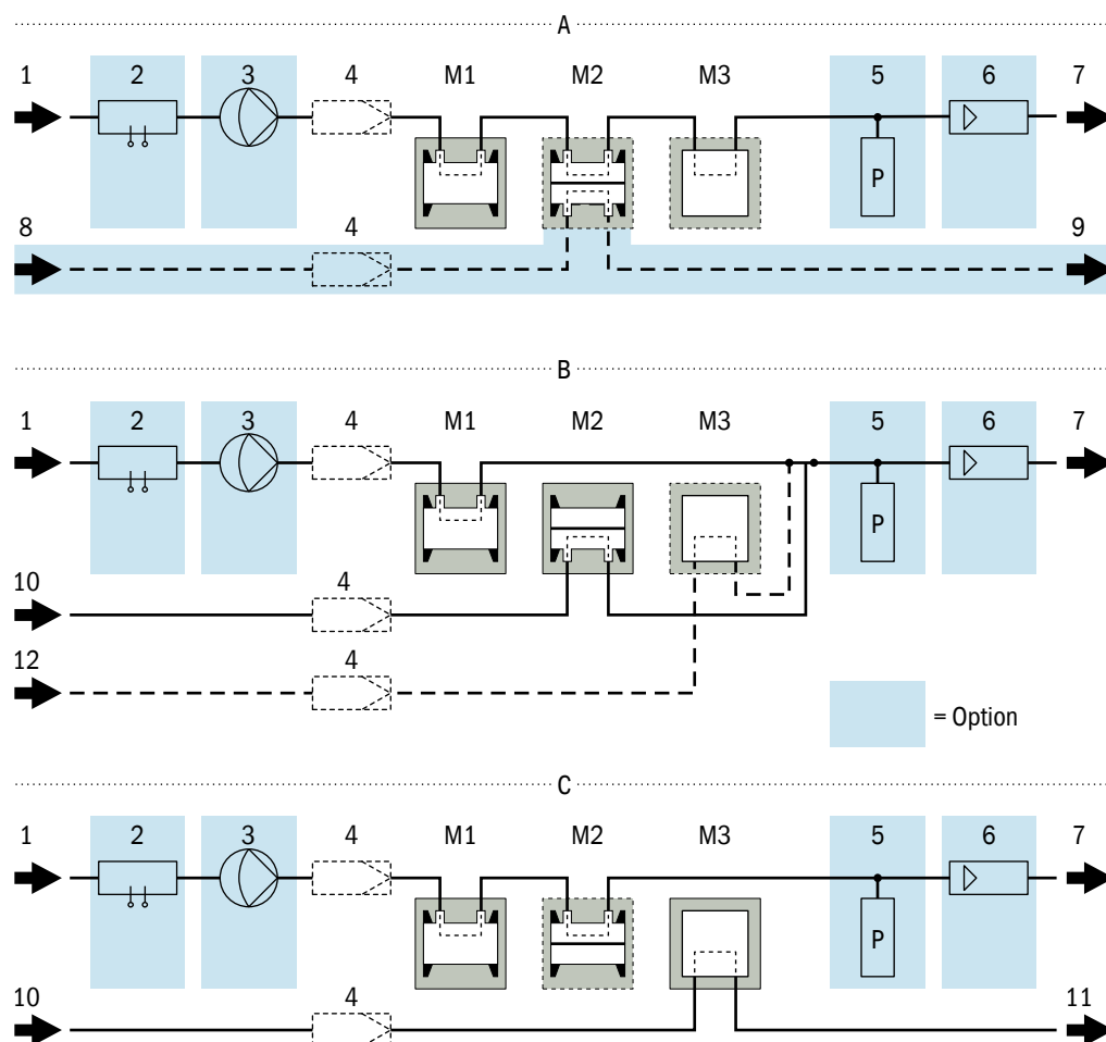
Fig. 40: Internal gas flow (standard flow schematics)
