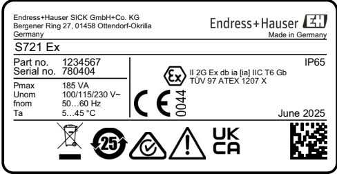
Fig. 7: Type plate S721 Ex (intrinsically safe)
