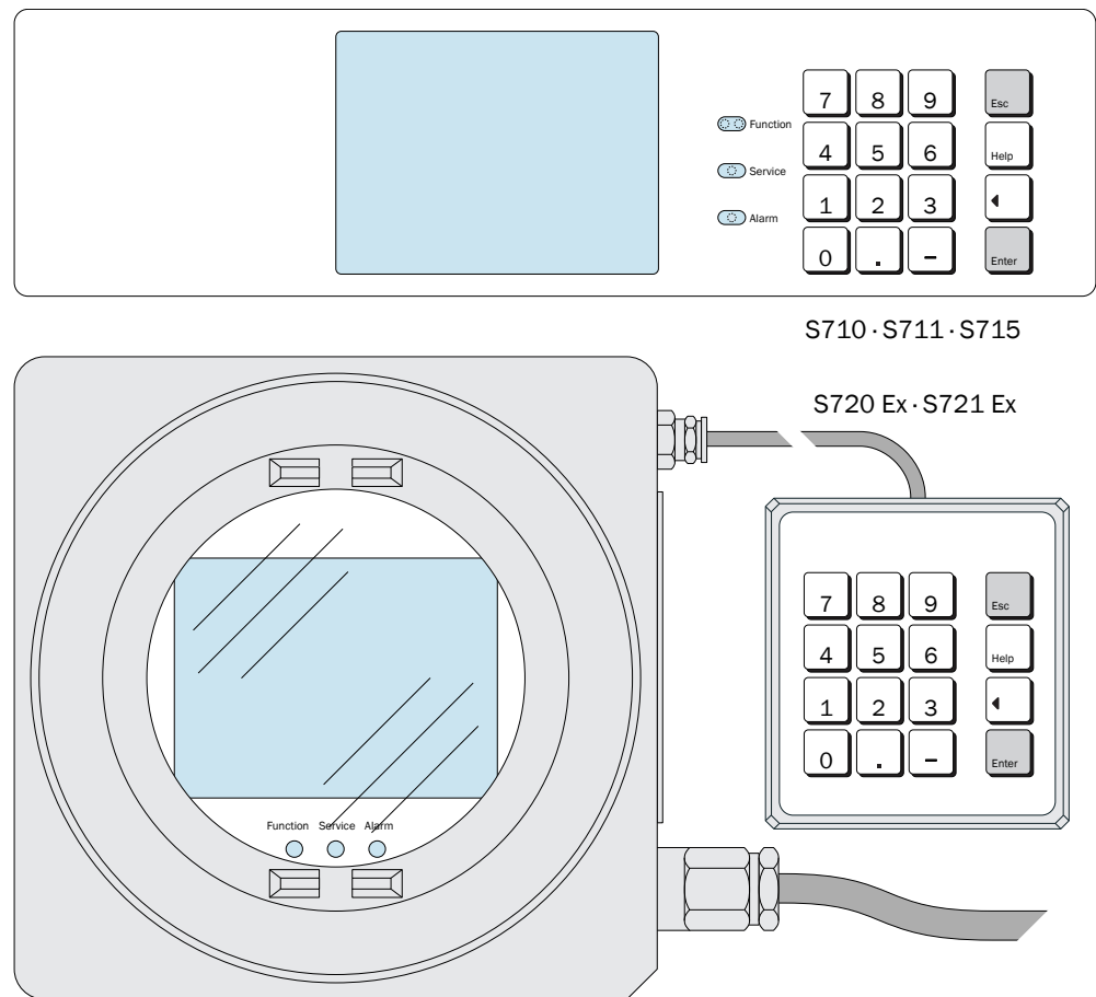
Fig. 26: Operating and display elements
