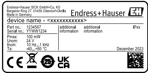
Fig. 3: Type plate S715 Ex
