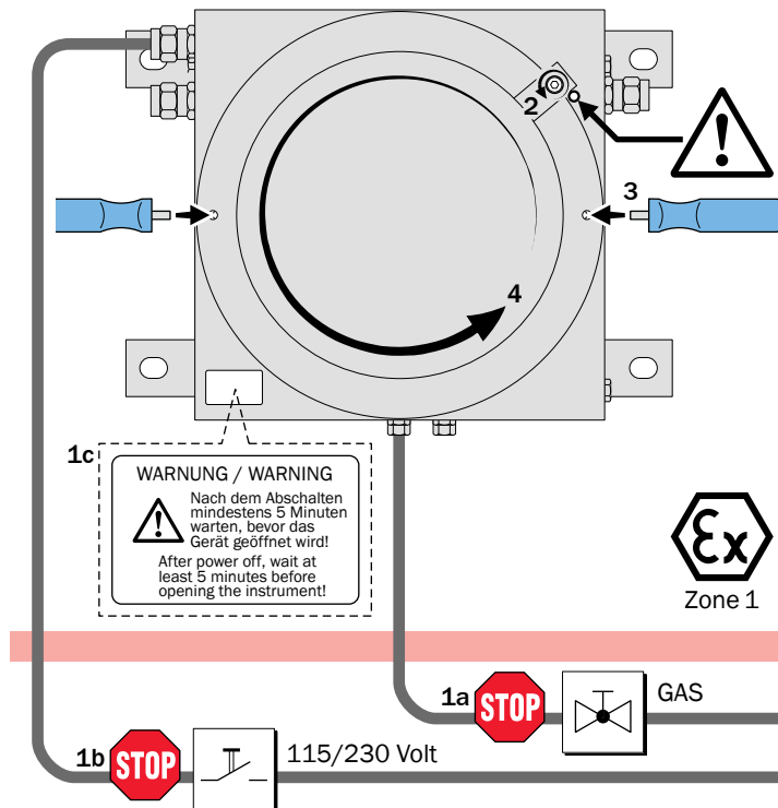
Fig. 12: Opening the analyzer enclosure for S720 Ex/S721 Ex
