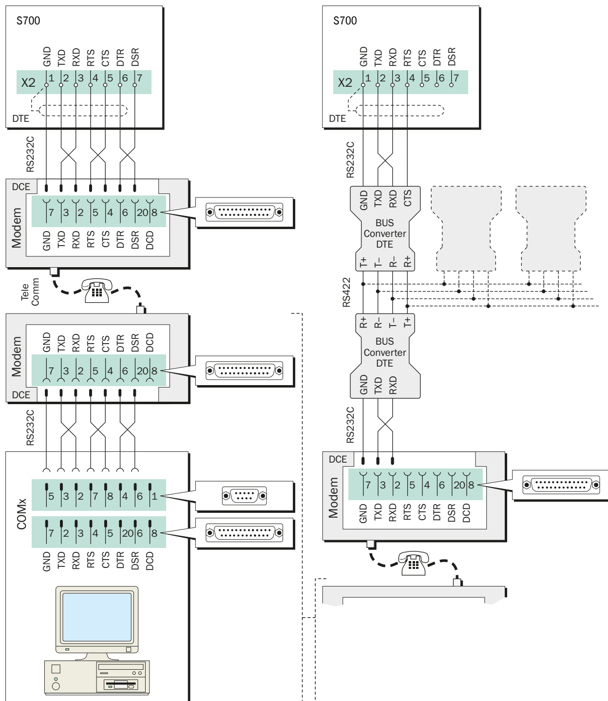
Fig. 35: Connection of gas analyzer and PC via modems
