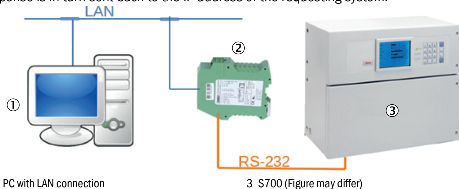
Fig. 2: Application case - Modbus TCP gateway
