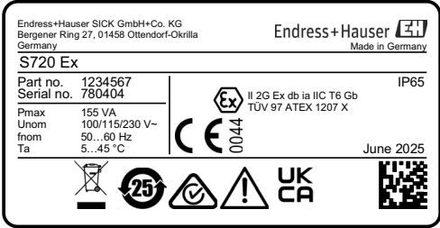
Fig. 5: Type plate S720 Ex (intrinsically safe)
