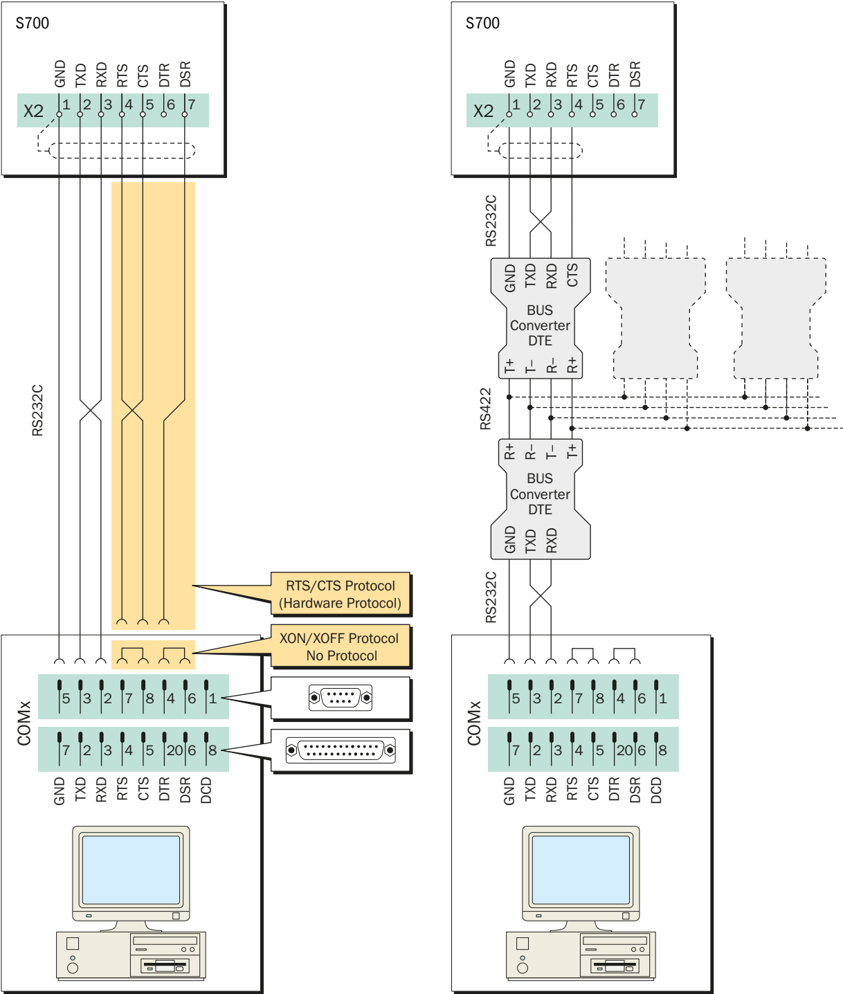
Fig. 34: Connection of gas analyzer and PC, without modems
