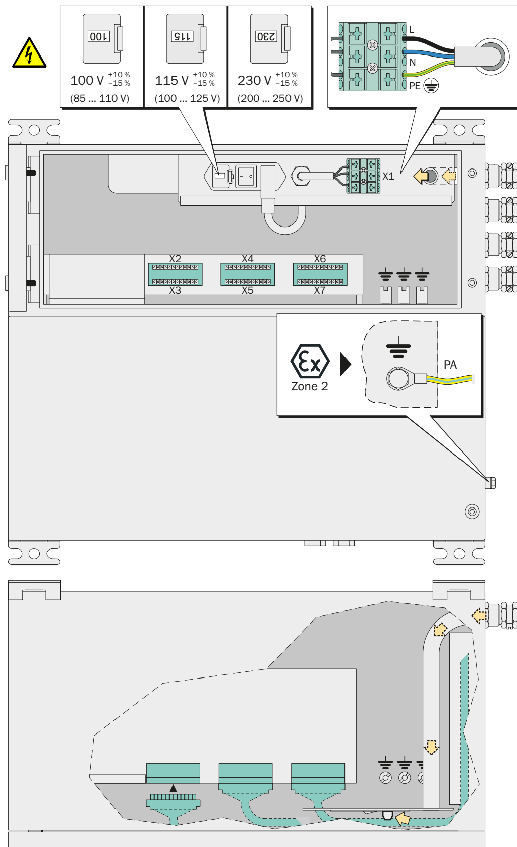
Fig. 15: S715 – power connection, position of the signal connections
