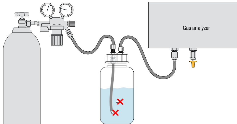
Fig. 30: A simple leak test method (example)
