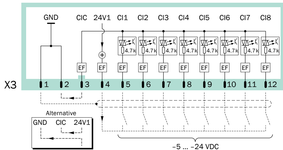
Fig. 23: Plug connector X3 (control inputs)
