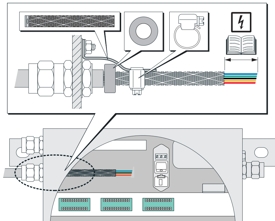
Fig. 13: Installation of signal cables for S720 Ex/S721 Ex
