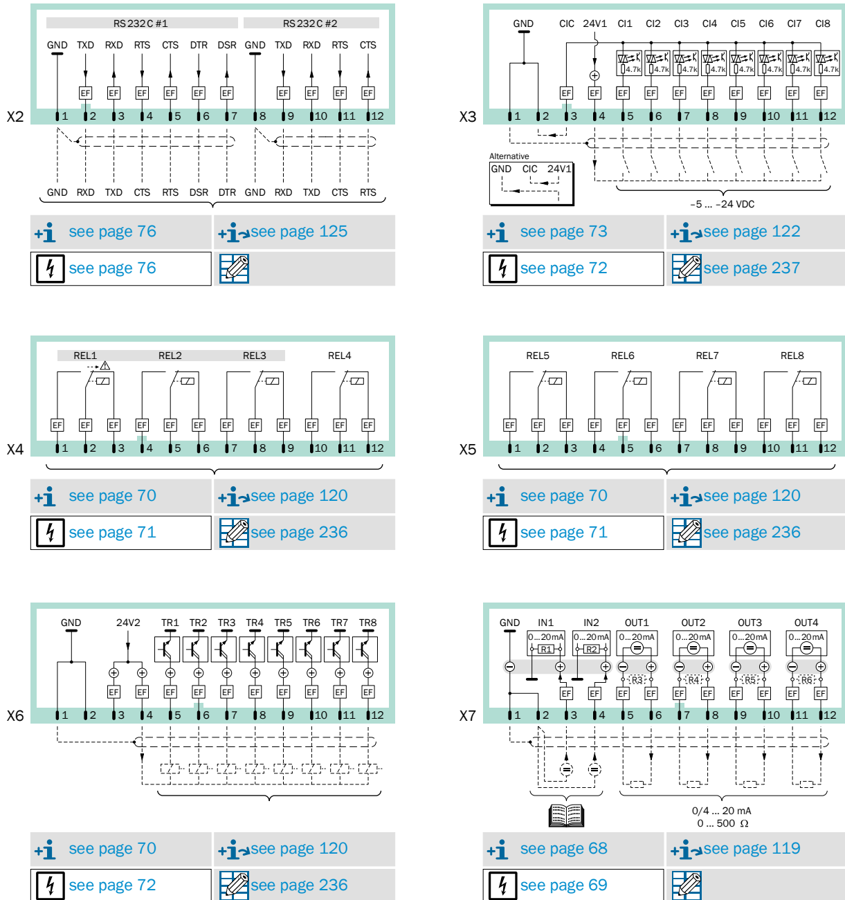
Fig. 36: Signal connection overview
