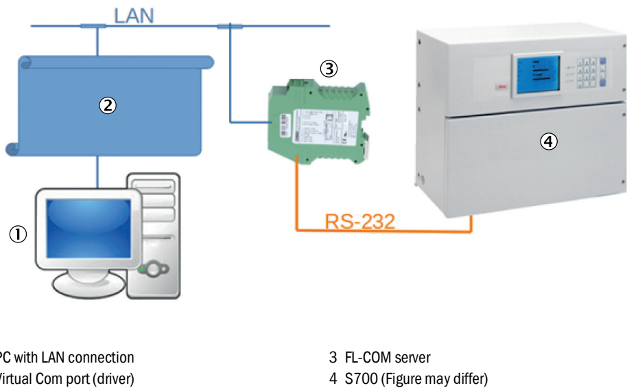
Fig. 1: Application case - Virtual serial interface
