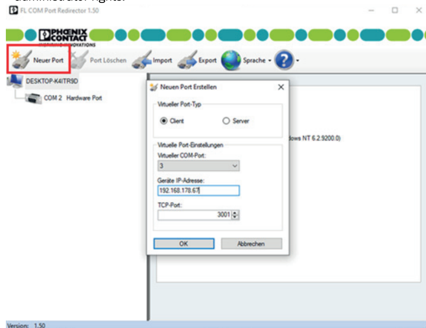
Fig. 18: Creating the virtual COM port
