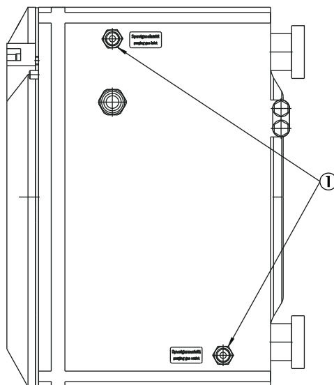
Fig. 10: Fitting options
