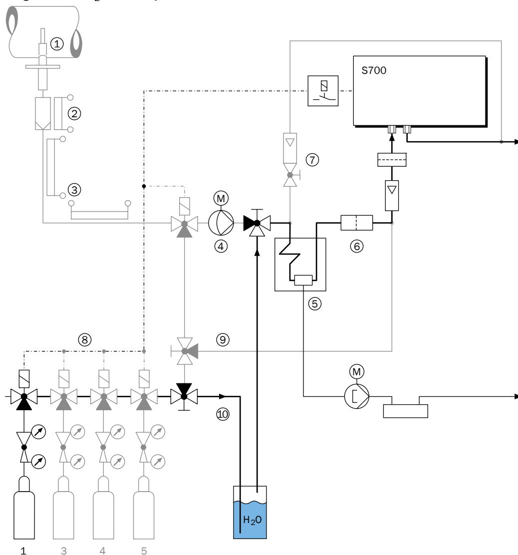
Fig. 29: Test gas feed for H 2 O sensitivity calibration
