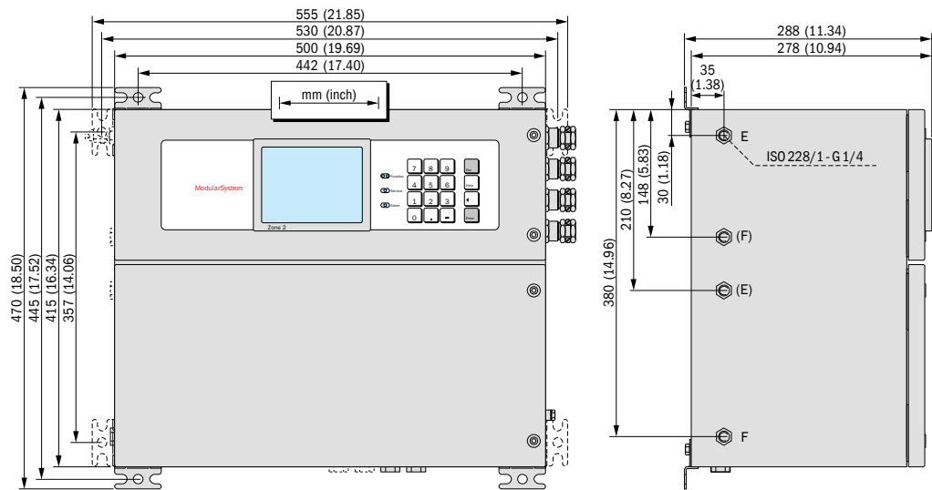
Fig. 38: Enclosure S715
