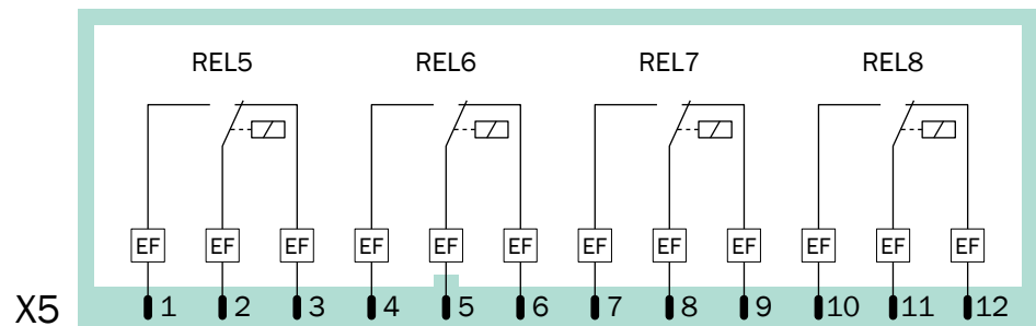
Fig. 21: Plug connector X5 (relay switching outputs)
