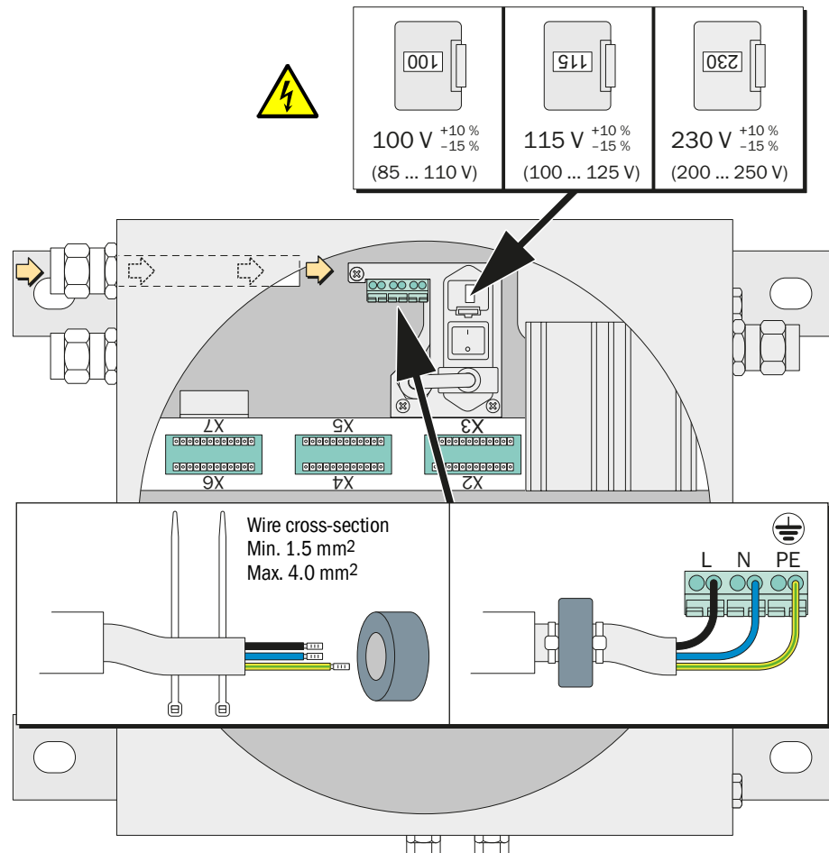
Fig. 16: S720 Ex/S721 Ex – power connection and position of the signal connections
