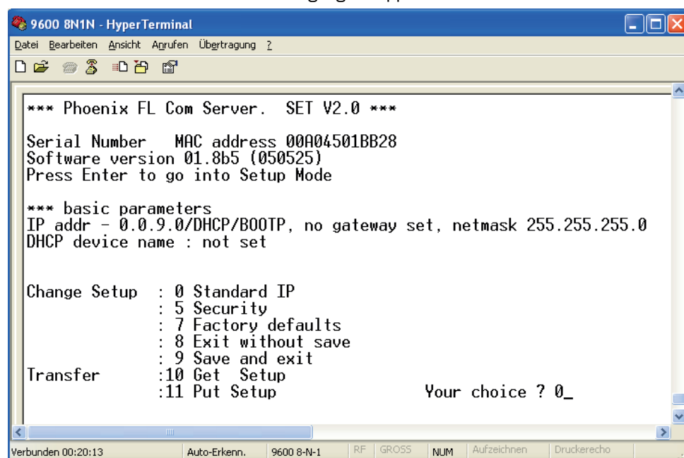
Fig. 23: Serial setup menu
