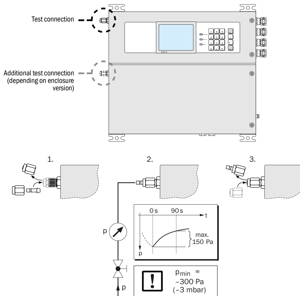
Fig. 31: Leak tightness check in Zone 2 for S715 Ex
