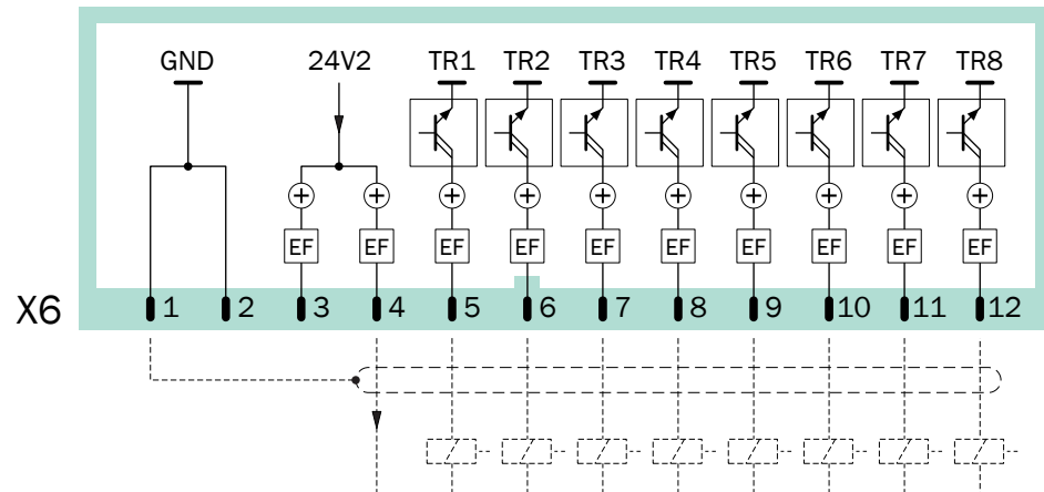
Fig. 22: Plug connector X6 (transistor switching outputs)
