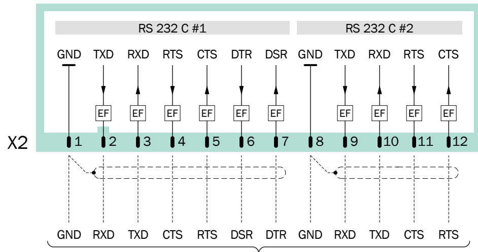
Fig. 25: Plug connector X2 (interfaces)
