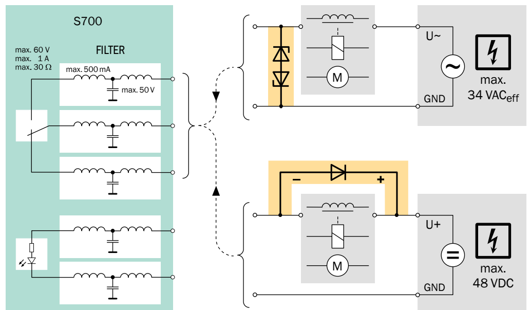
Fig. 18: Connecting inductive loads
