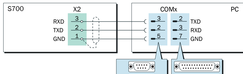
Fig. 28: Minimum interface connection for the program loader function
