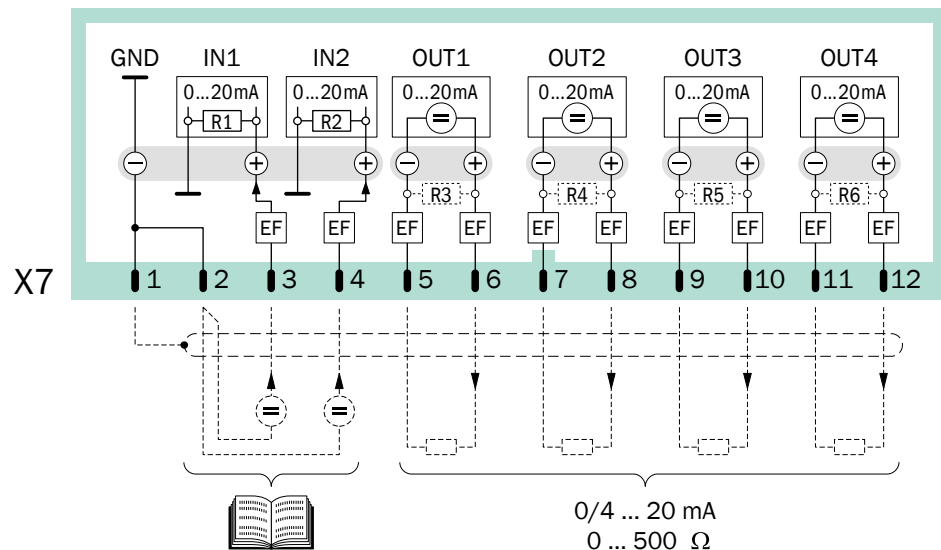
Fig. 19: Plug connector X7 (analog inputs, measured value outputs)
