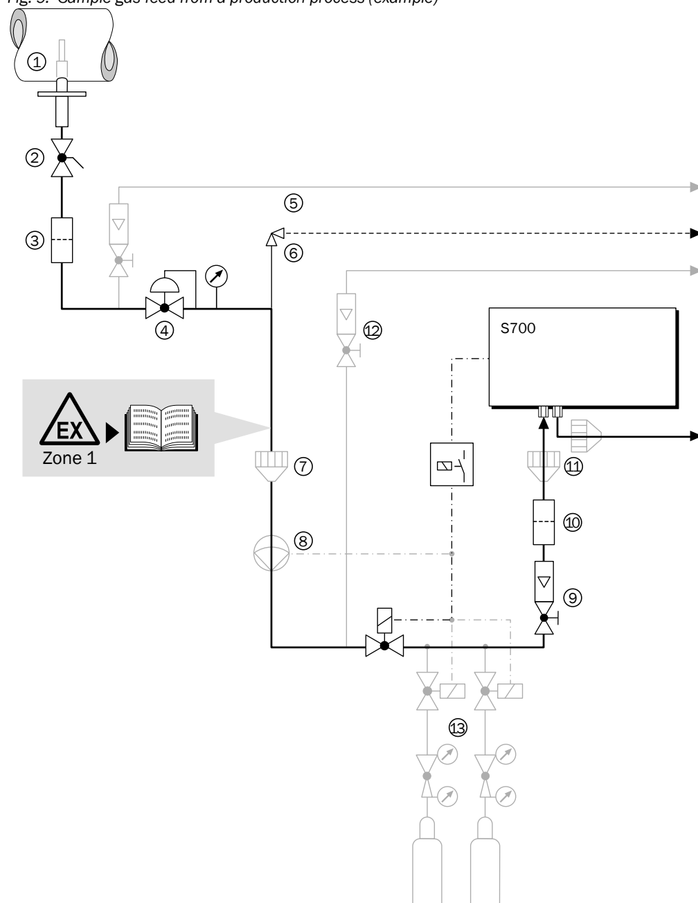
Fig. 9: Sample gas feed from a production process (example)
