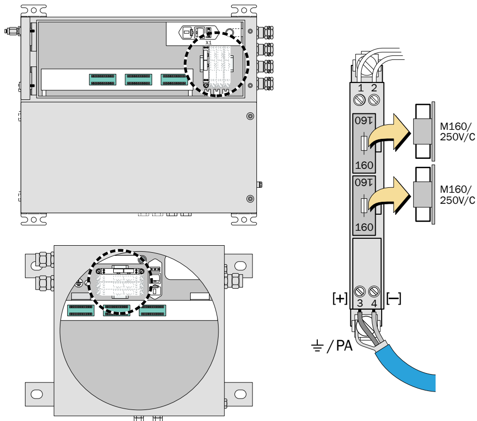
Fig. 24: Intrinsically-safe measured value outputs
