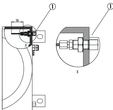
Fig. 11: Fitting details
