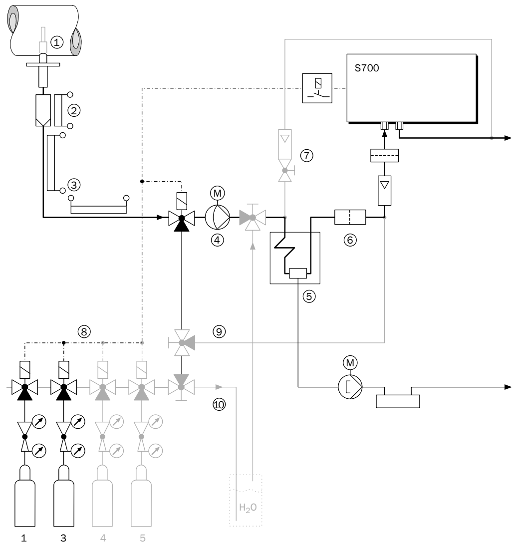
Fig. 8: Sample gas feed from an emission source (example)
