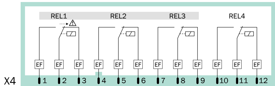
Fig. 20: Plug connector X4 (relay switching outputs)
