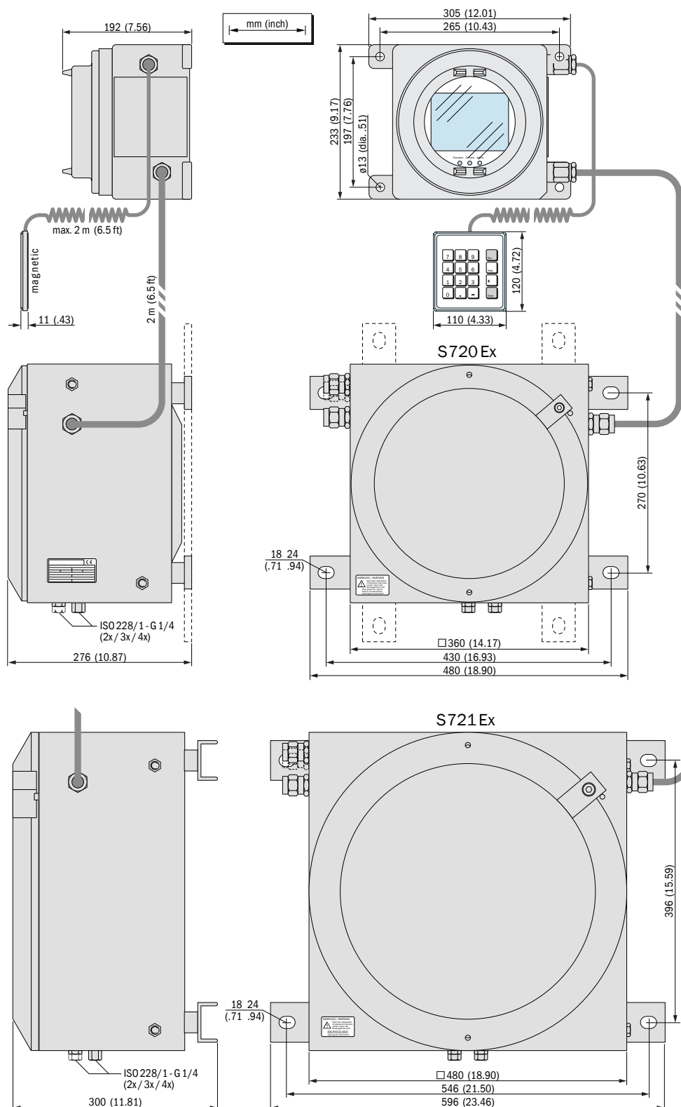
Fig. 39: Enclosure S720 Ex/S721 Ex
