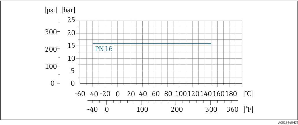
25 Process connection material: stainless steel, 1.4404 (F316L)
