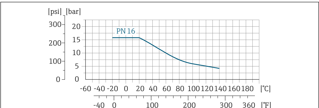
19 Process connection material: PVDF
