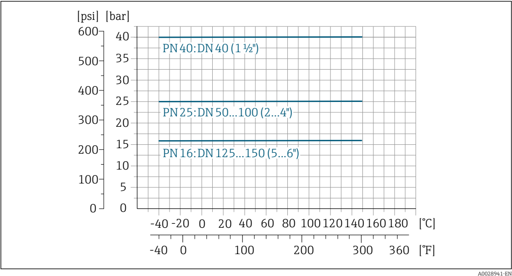
27 Process connection material: stainless steel, 1.4404 (F316L)
