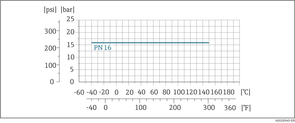
26 Process connection material: stainless steel, 1.4404 (F316L)
