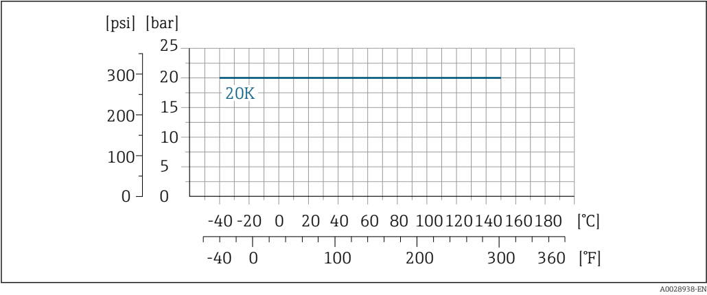
23 Process connection material: stainless steel, 1.4404 (F316L)
