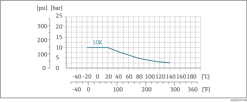
24 Process connection material: PVDF
