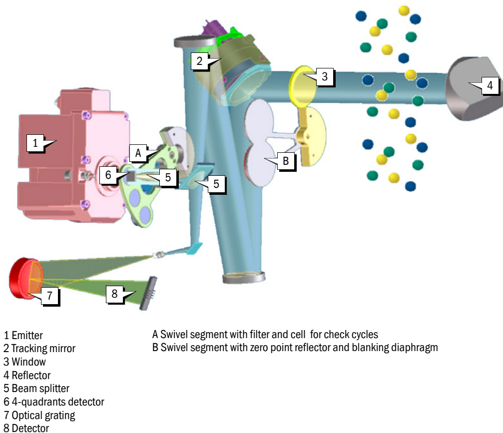
Fig. 1 Measuring principle
