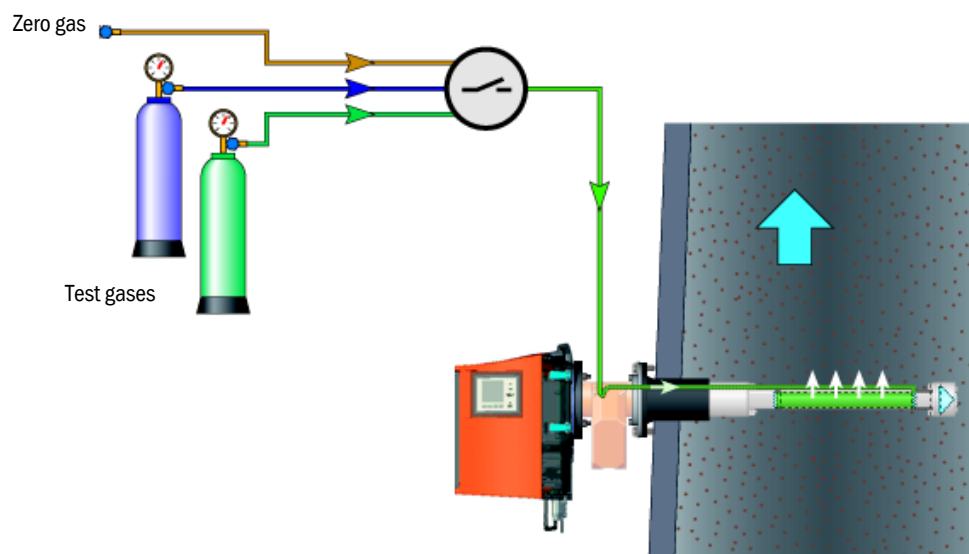
Fig. 15 Test gas measurement with GPP probe
