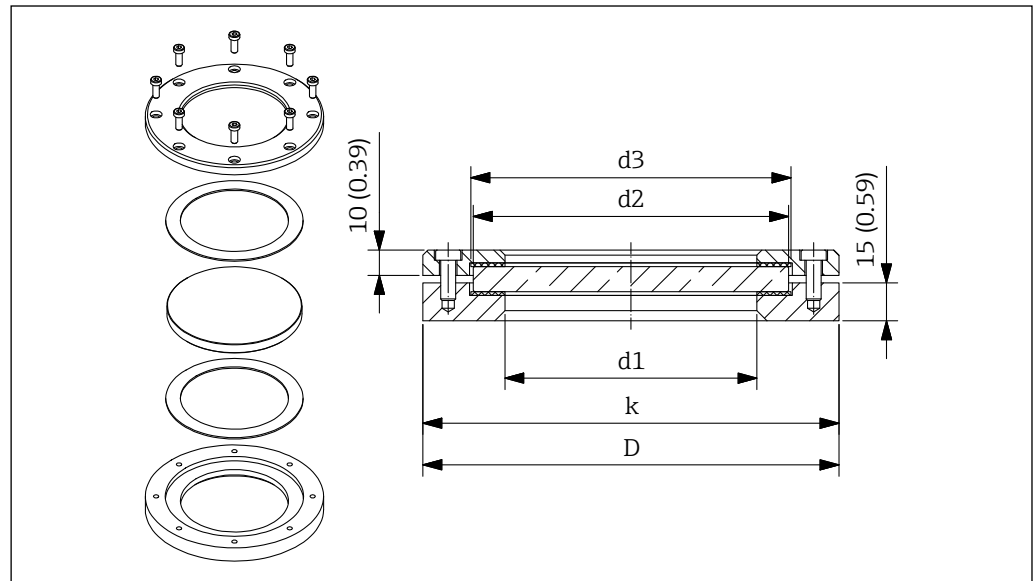
34 Dimensions sight glass fitting for unpressurized processes. Unit of measurement mm (in)
