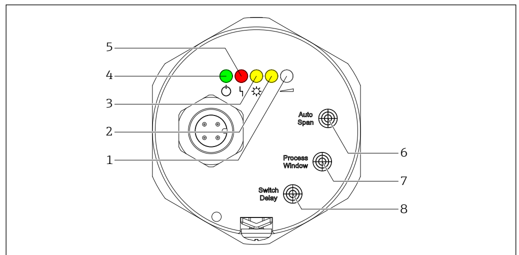
19 Display and operating elements of the FTR16
