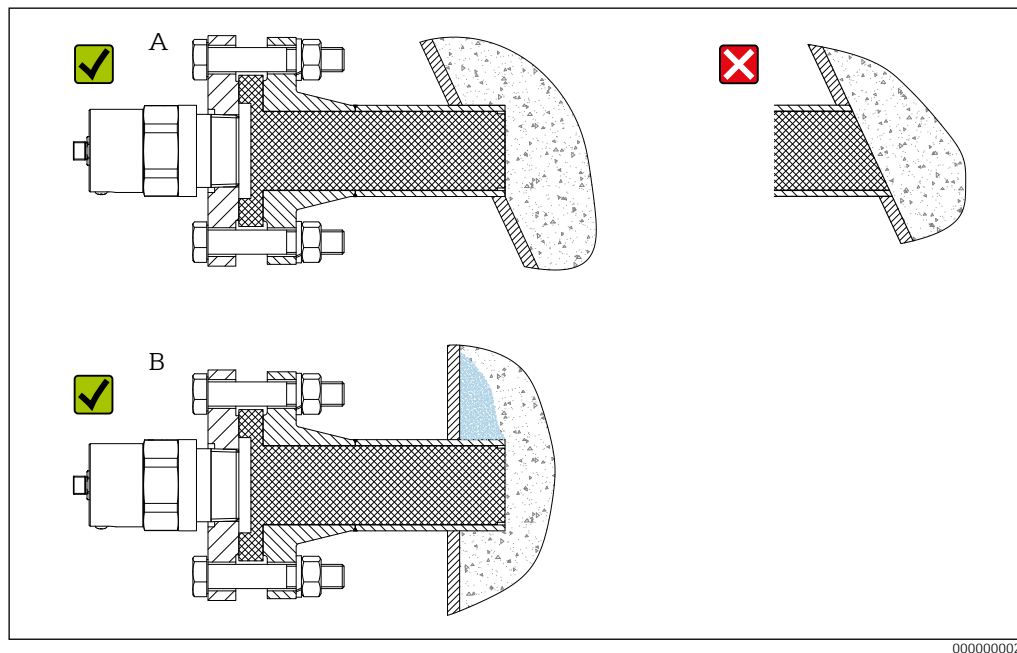
12 Mounting with risk of buildup
